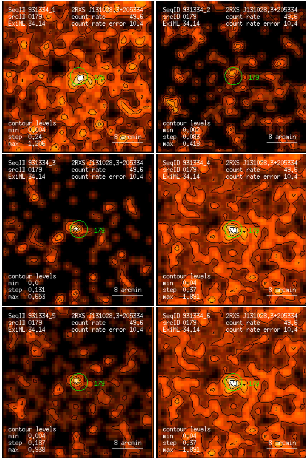
Figure 179: RASS 931334: detection 0179: band rate images, Gaussian filter: (1) PSPC channels 11 – 41, (2) 52 – 90, (3) 91 – 201, (4) 11 – 235, (5) 52 – 201, (6) 11 – 201. Broad band rates in counts/ks. Band rate contour levels in counts/ks/arcmin 2 .
