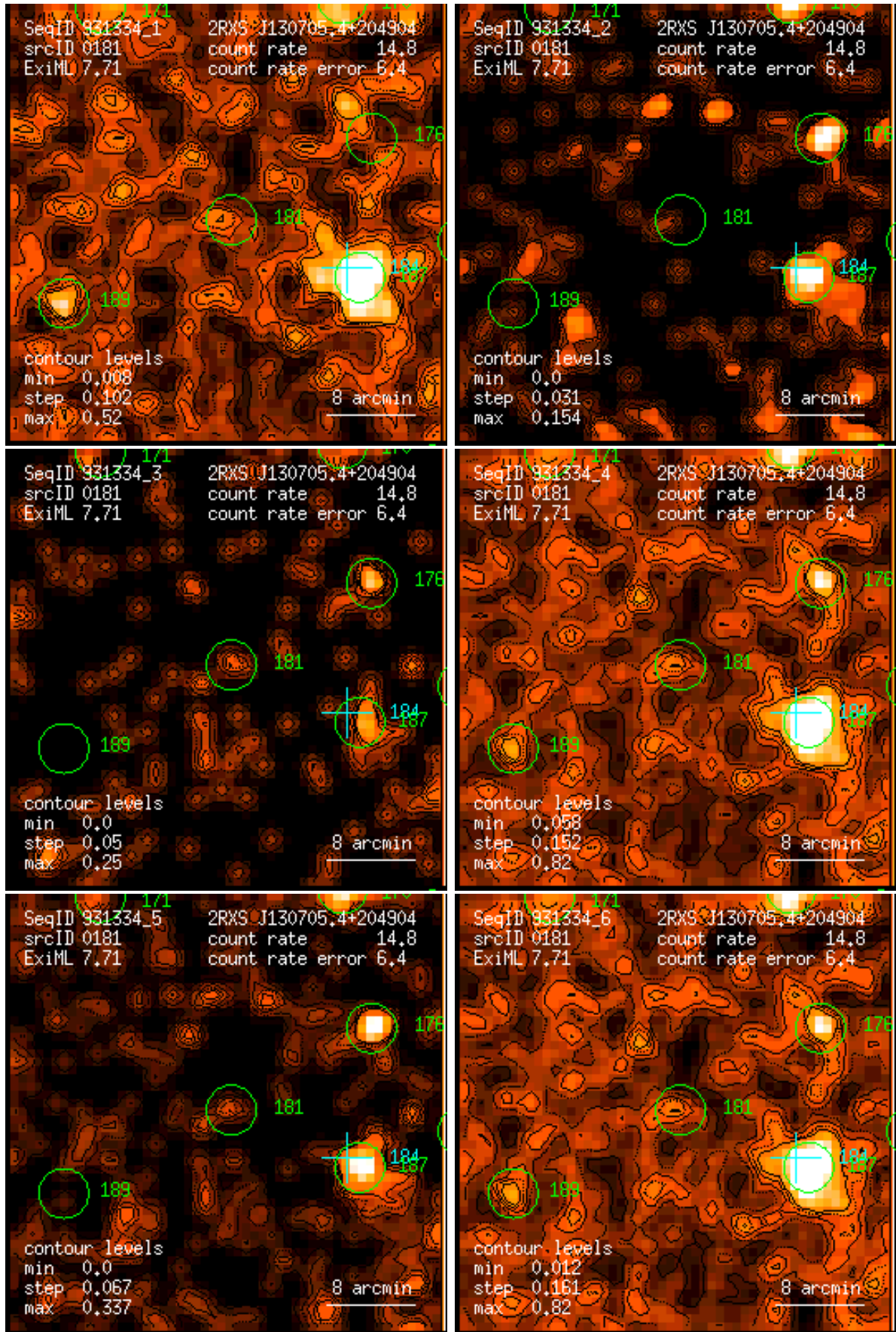
Figure 181: RASS 931334: detection 0181: band rate images, Gaussian filter: (1) PSPC channels 11 – 41, (2) 52 – 90, (3) 91 – 201, (4) 11 – 235, (5) 52 – 201, (6) 11 – 201. Broad band rates in counts/ks. Band rate contour levels in counts/ks/arcmin 2 .
