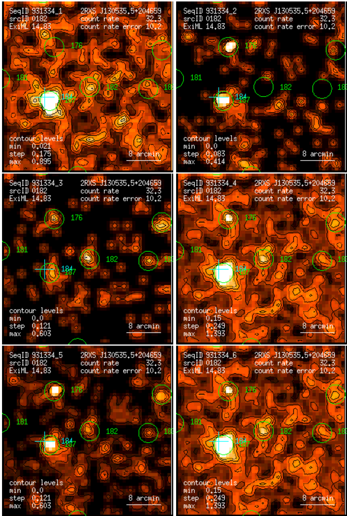
Figure 182: RASS 931334: detection 0182: band rate images, Gaussian filter: (1) PSPC channels 11 – 41, (2) 52 – 90, (3) 91 – 201, (4) 11 – 235, (5) 52 – 201, (6) 11 – 201. Broad band rates in counts/ks. Band rate contour levels in counts/ks/arcmin 2 .
