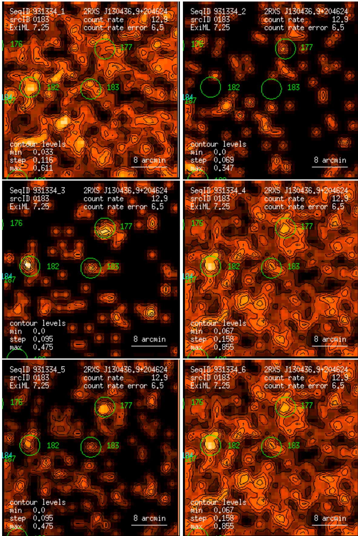
Figure 183: RASS 931334: detection 0183: band rate images, Gaussian filter: (1) PSPC channels 11 – 41, (2) 52 – 90, (3) 91 – 201, (4) 11 – 235, (5) 52 – 201, (6) 11 – 201. Broad band rates in counts/ks. Band rate contour levels in counts/ks/arcmin 2 .
