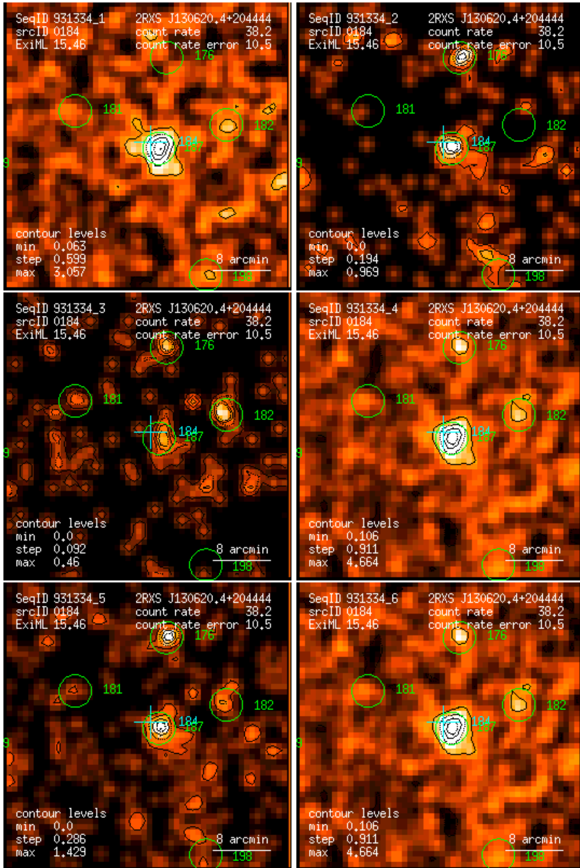
Figure 184: RASS 931334: detection 0184: band rate images, Gaussian filter: (1) PSPC channels 11 – 41, (2) 52 – 90, (3) 91 – 201, (4) 11 – 235, (5) 52 – 201, (6) 11 – 201. Broad band rates in counts/ks. Band rate contour levels in counts/ks/arcmin 2 .
