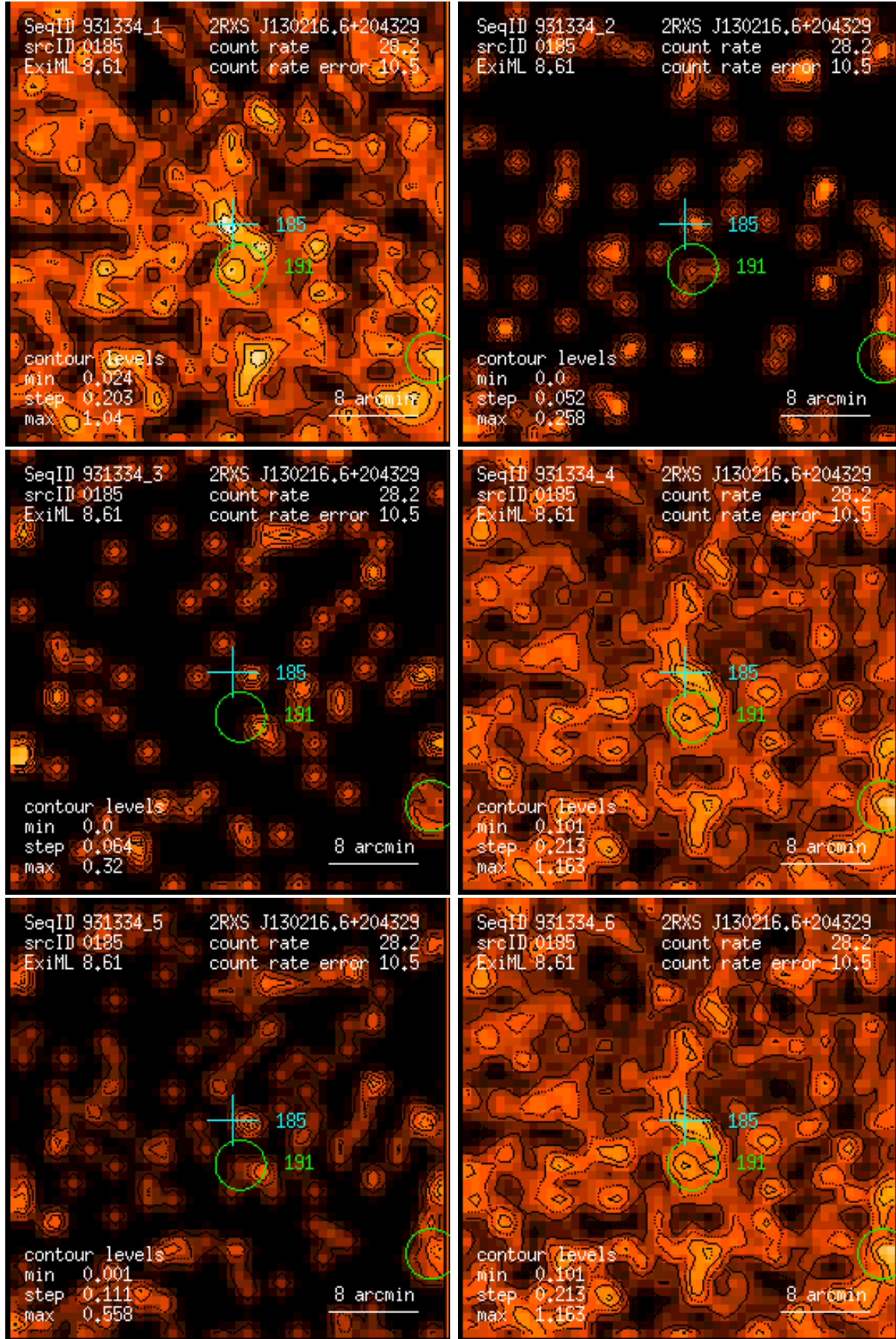
Figure 185: RASS 931334: detection 0185: band rate images, Gaussian filter: (1) PSPC channels 11 – 41, (2) 52 – 90, (3) 91 – 201, (4) 11 – 235, (5) 52 – 201, (6) 11 – 201. Broad band rates in counts/ks. Band rate contour levels in counts/ks/arcmin 2 .
