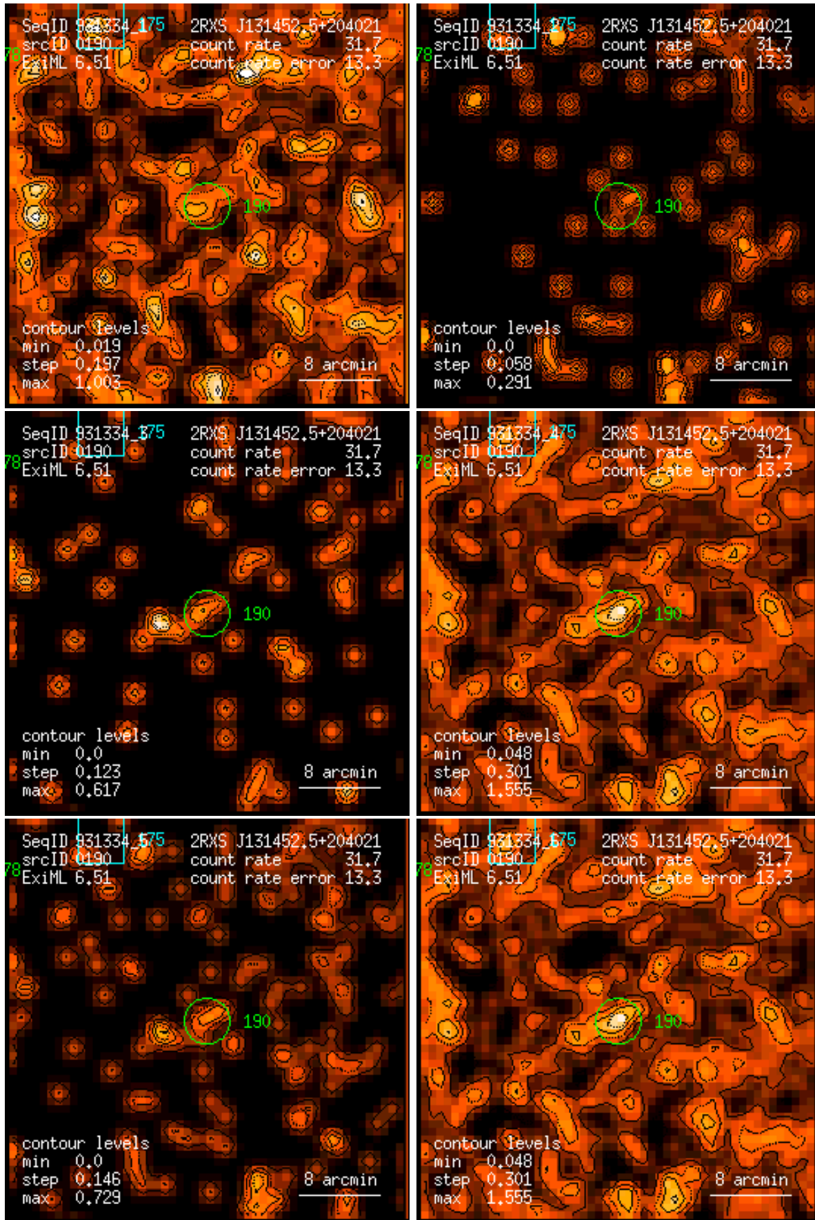
Figure 190: RASS 931334: detection 0190: band rate images, Gaussian filter: (1) PSPC channels 11 – 41, (2) 52 – 90, (3) 91 – 201, (4) 11 – 235, (5) 52 – 201, (6) 11 – 201. Broad band rates in counts/ks. Band rate contour levels in counts/ks/arcmin 2 .
