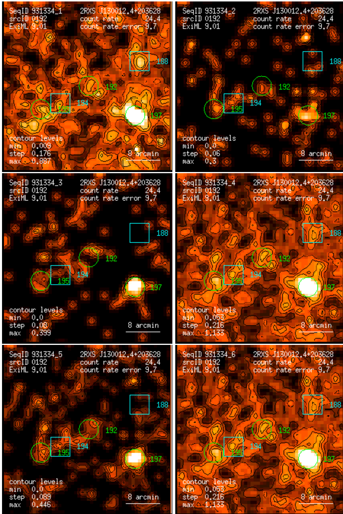
Figure 192: RASS 931334: detection 0192: band rate images, Gaussian filter: (1) PSPC channels 11 – 41, (2) 52 – 90, (3) 91 – 201, (4) 11 – 235, (5) 52 – 201, (6) 11 – 201. Broad band rates in counts/ks. Band rate contour levels in counts/ks/arcmin 2 .
