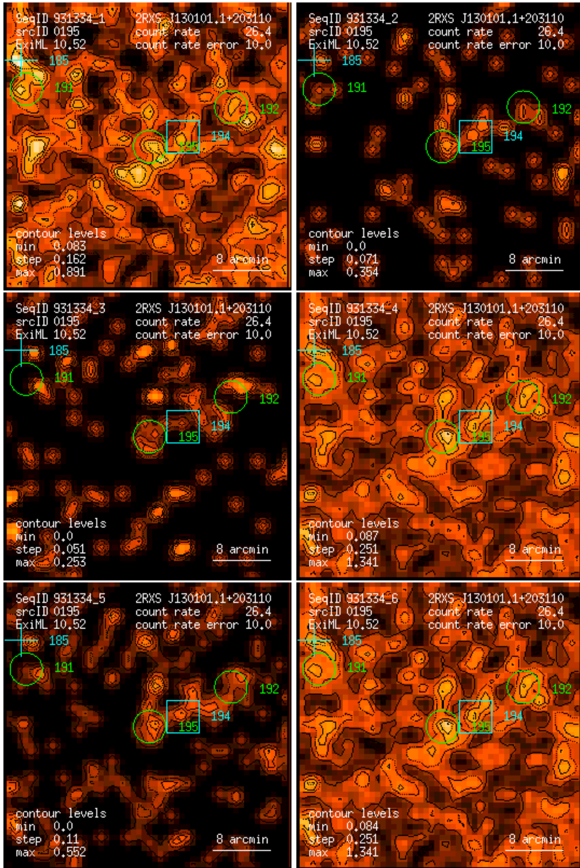
Figure 195: RASS 931334: detection 0195: band rate images, Gaussian filter: (1) PSPC channels 11 – 41, (2) 52 – 90, (3) 91 – 201, (4) 11 – 235, (5) 52 – 201, (6) 11 – 201. Broad band rates in counts/ks. Band rate contour levels in counts/ks/arcmin 2 .
