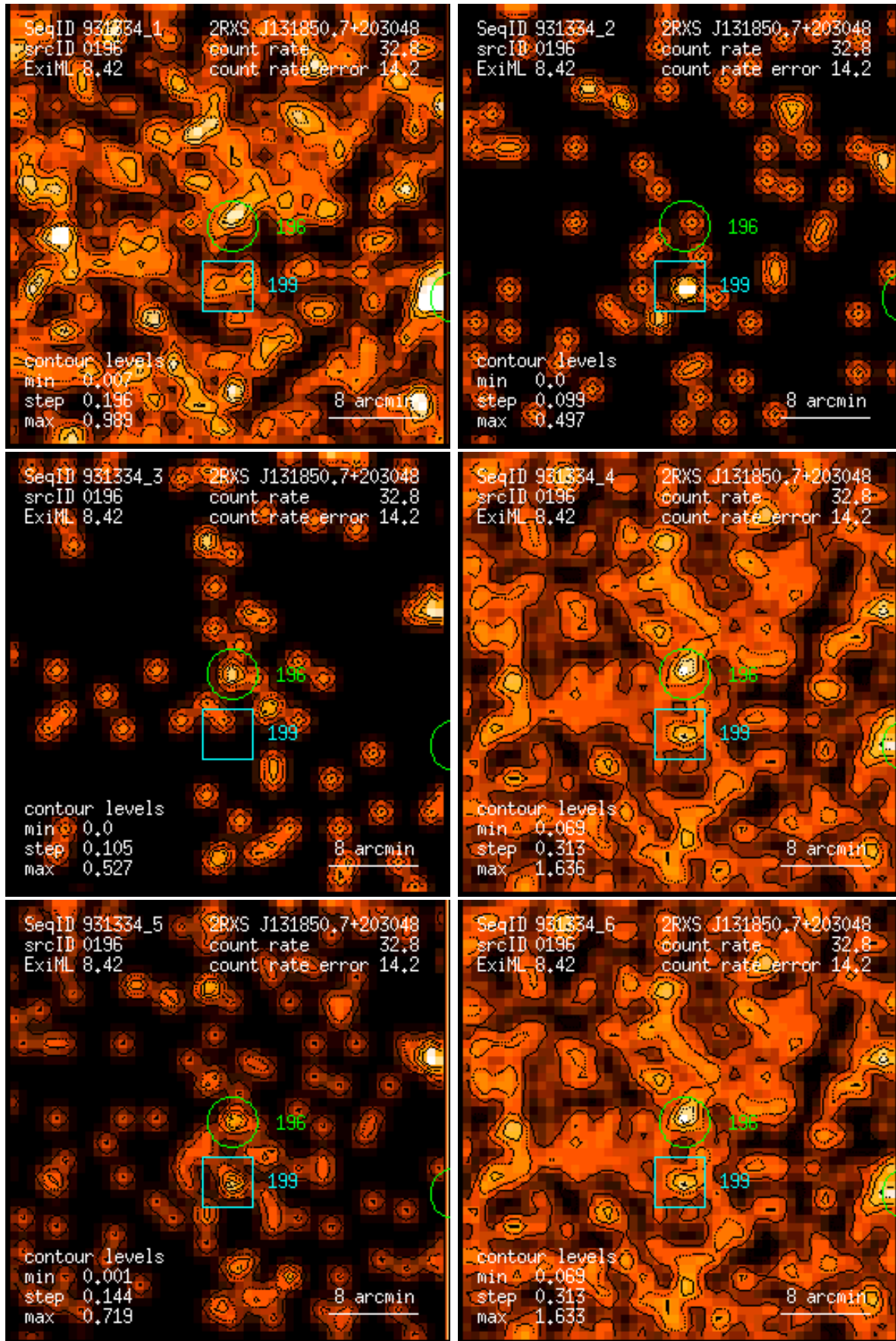
Figure 196: RASS 931334: detection 0196: band rate images, Gaussian filter: (1) PSPC channels 11 – 41, (2) 52 – 90, (3) 91 – 201, (4) 11 – 235, (5) 52 – 201, (6) 11 – 201. Broad band rates in counts/ks. Band rate contour levels in counts/ks/arcmin 2 .
