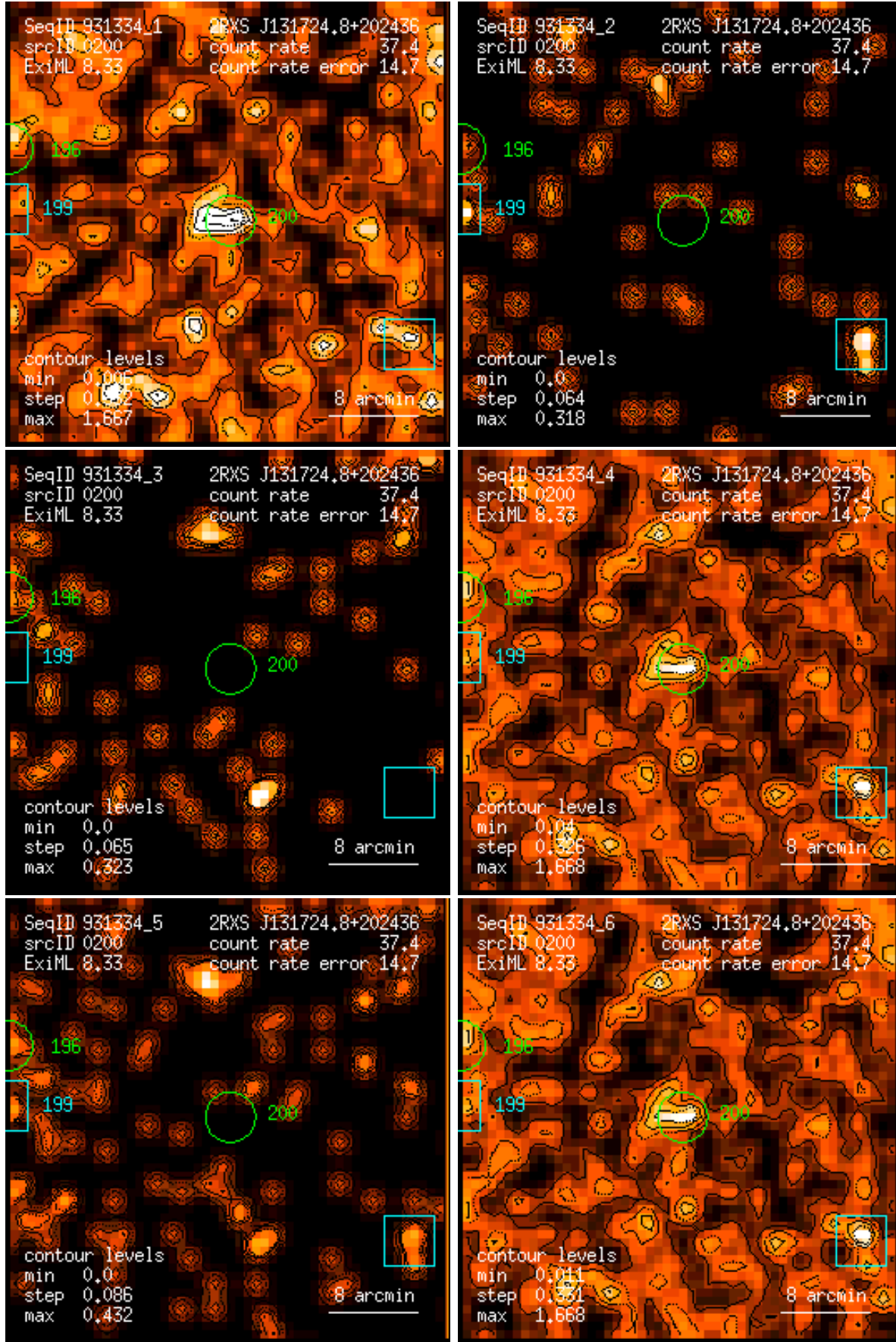
Figure 200: RASS 931334: detection 0200: band rate images, Gaussian filter: (1) PSPC channels 11 – 41, (2) 52 – 90, (3) 91 – 201, (4) 11 – 235, (5) 52 – 201, (6) 11 – 201. Broad band rates in counts/ks. Band rate contour levels in counts/ks/arcmin 2 .
