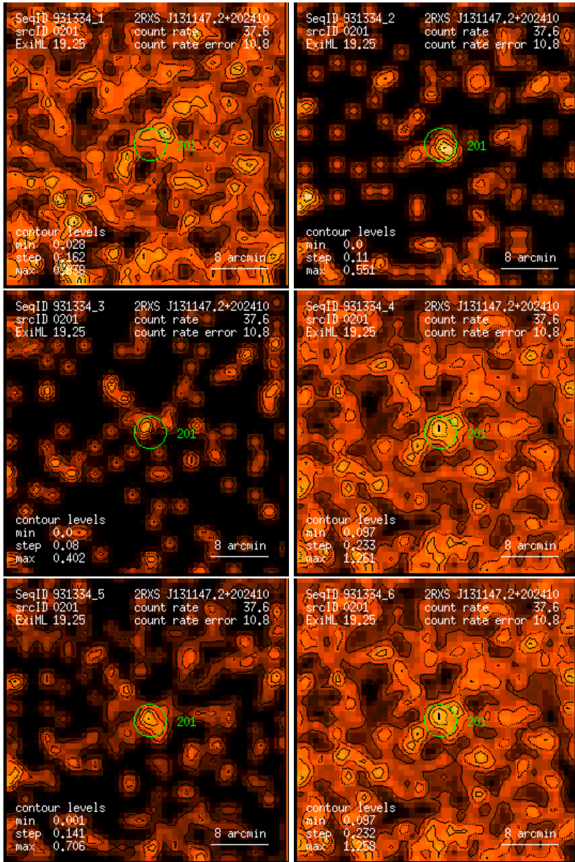
Figure 201: RASS 931334: detection 0201: band rate images, Gaussian filter: (1) PSPC channels 11 – 41, (2) 52 – 90, (3) 91 – 201, (4) 11 – 235, (5) 52 – 201, (6) 11 – 201. Broad band rates in counts/ks. Band rate contour levels in counts/ks/arcmin 2 .
