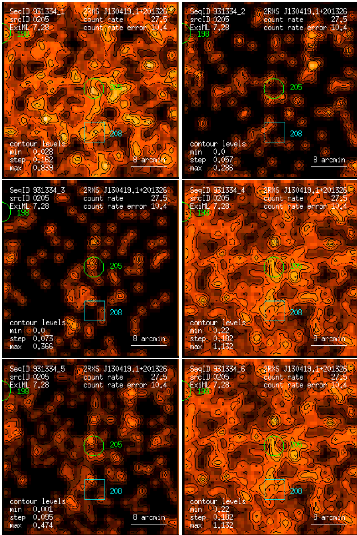
Figure 205: RASS 931334: detection 0205: band rate images, Gaussian filter: (1) PSPC channels 11 – 41, (2) 52 – 90, (3) 91 – 201, (4) 11 – 235, (5) 52 – 201, (6) 11 – 201. Broad band rates in counts/ks. Band rate contour levels in counts/ks/arcmin 2 .
