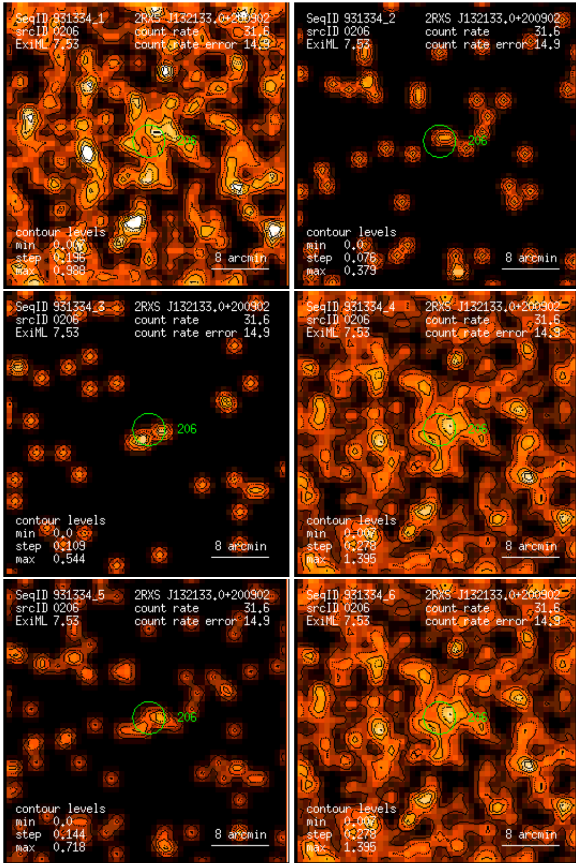
Figure 206: RASS 931334: detection 0206: band rate images, Gaussian filter: (1) PSPC channels 11 – 41, (2) 52 – 90, (3) 91 – 201, (4) 11 – 235, (5) 52 – 201, (6) 11 – 201. Broad band rates in counts/ks. Band rate contour levels in counts/ks/arcmin 2 .
