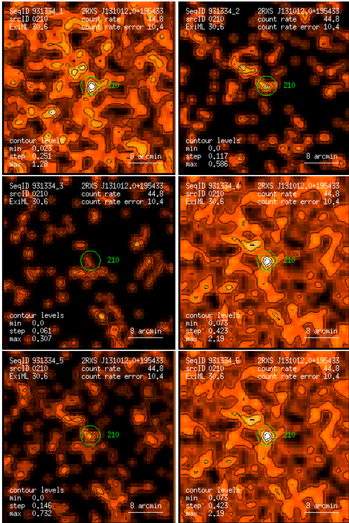
Figure 210: RASS 931334: detection 0210: band rate images, Gaussian filter: (1) PSPC channels 11 – 41, (2) 52 – 90, (3) 91 – 201, (4) 11 – 235, (5) 52 – 201, (6) 11 – 201. Broad band rates in counts/ks. Band rate contour levels in counts/ks/arcmin 2 .
