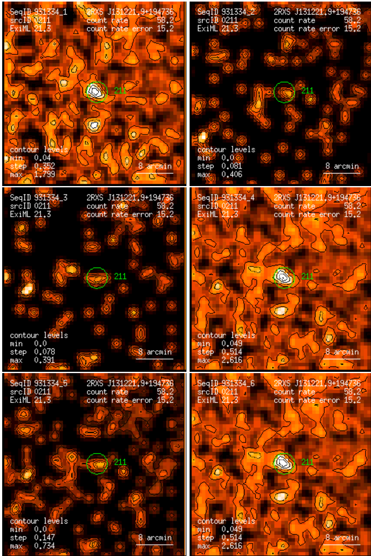
Figure 211: RASS 931334: detection 0211: band rate images, Gaussian filter: (1) PSPC channels 11 – 41, (2) 52 – 90, (3) 91 – 201, (4) 11 – 235, (5) 52 – 201, (6) 11 – 201. Broad band rates in counts/ks. Band rate contour levels in counts/ks/arcmin 2 .
