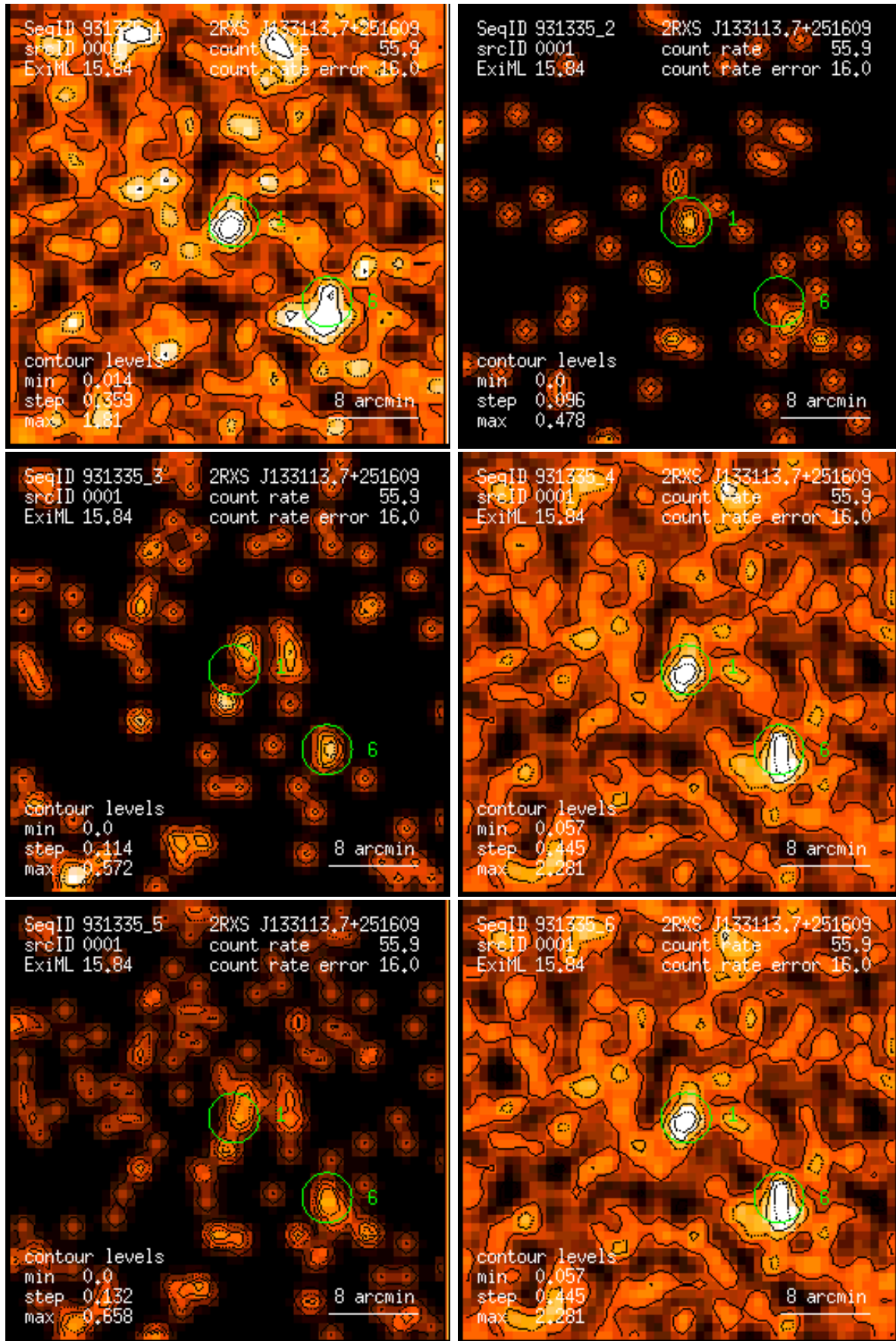
Figure 1: RASS 931335: detection 0001: band rate images, Gaussian filter: (1) PSPC channels 11 – 41, (2) 52 – 90, (3) 91 – 201, (4) 11 – 235, (5) 52 – 201, (6) 11 – 201. Broad band rates in counts/ks. Band rate contour levels in counts/ks/arcmin 2 .
