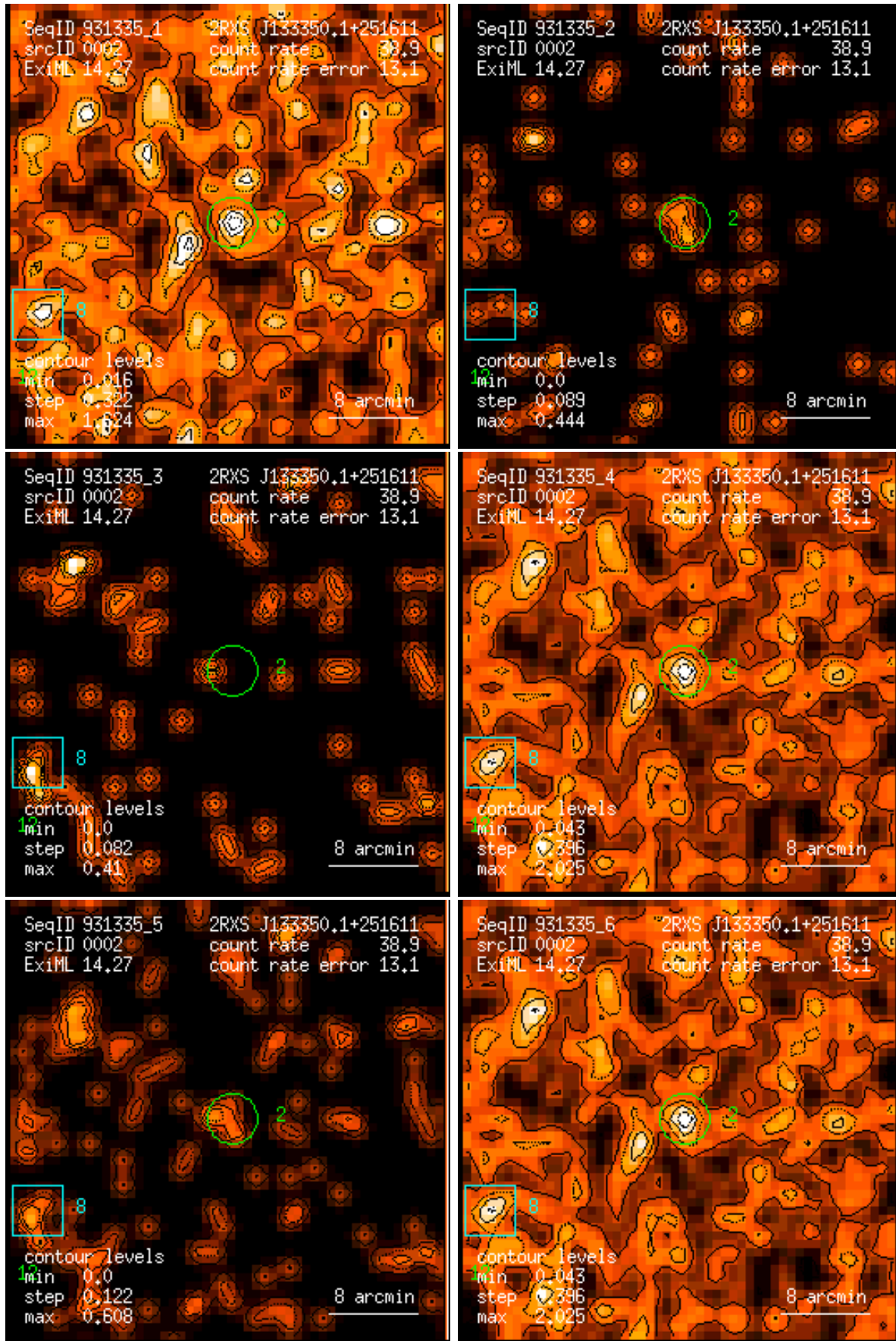
Figure 2: RASS 931335: detection 0002: band rate images, Gaussian filter: (1) PSPC channels 11 – 41, (2) 52 – 90, (3) 91 – 201, (4) 11 – 235, (5) 52 – 201, (6) 11 – 201. Broad band rates in counts/ks. Band rate contour levels in counts/ks/arcmin 2 .
