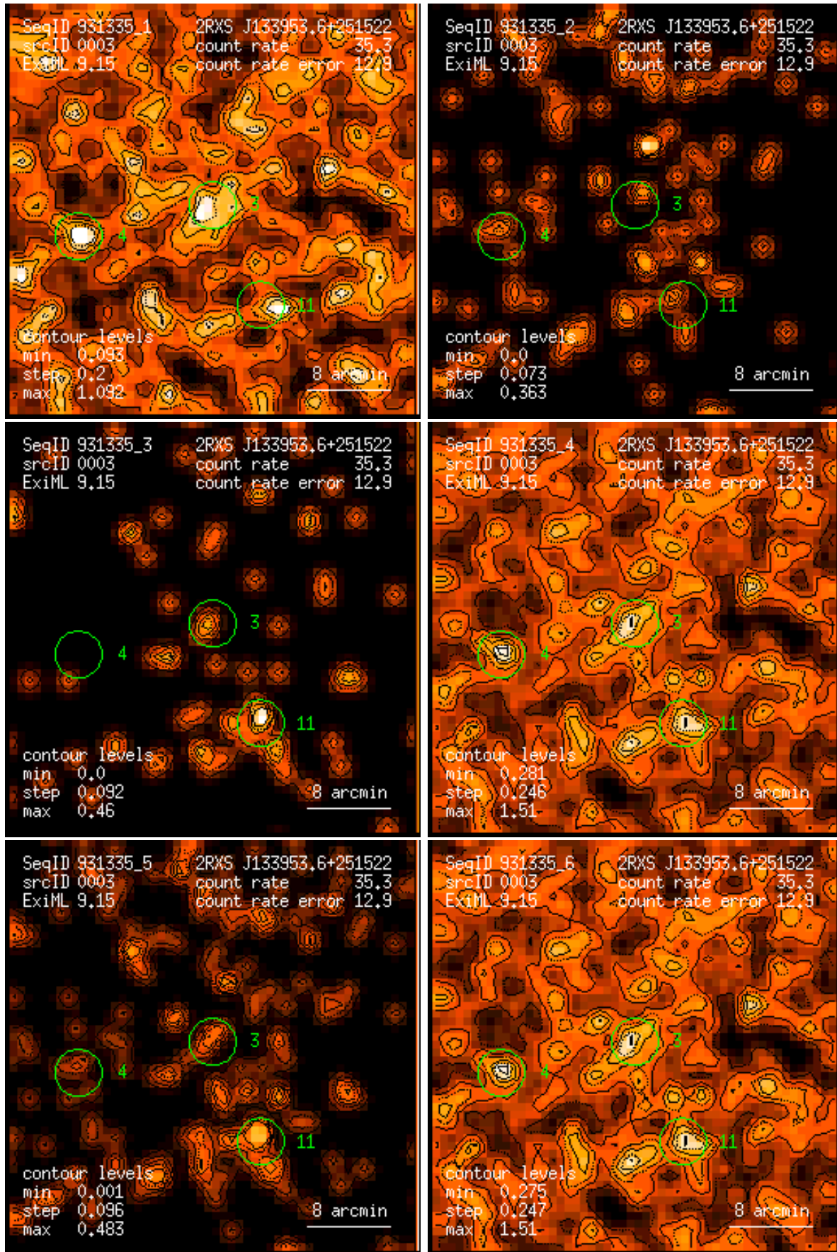
Figure 3: RASS 931335: detection 0003: band rate images, Gaussian filter: (1) PSPC channels 11 – 41, (2) 52 – 90, (3) 91 – 201, (4) 11 – 235, (5) 52 – 201, (6) 11 – 201. Broad band rates in counts/ks. Band rate contour levels in counts/ks/arcmin 2 .
