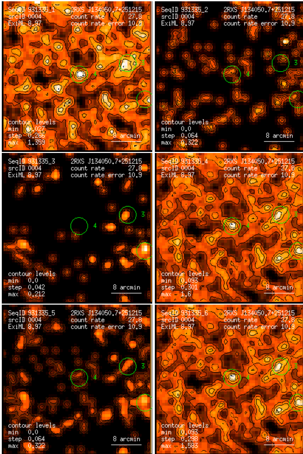
Figure 4: RASS 931335: detection 0004: band rate images, Gaussian filter: (1) PSPC channels 11 – 41, (2) 52 – 90, (3) 91 – 201, (4) 11 – 235, (5) 52 – 201, (6) 11 – 201. Broad band rates in counts/ks. Band rate contour levels in counts/ks/arcmin 2 .
