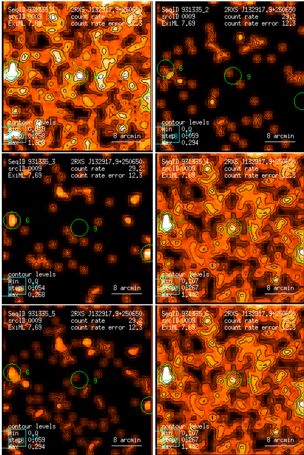
Figure 9: RASS 931335: detection 0009: band rate images, Gaussian filter: (1) PSPC channels 11 – 41, (2) 52 – 90, (3) 91 – 201, (4) 11 – 235, (5) 52 – 201, (6) 11 – 201. Broad band rates in counts/ks. Band rate contour levels in counts/ks/arcmin 2 .
