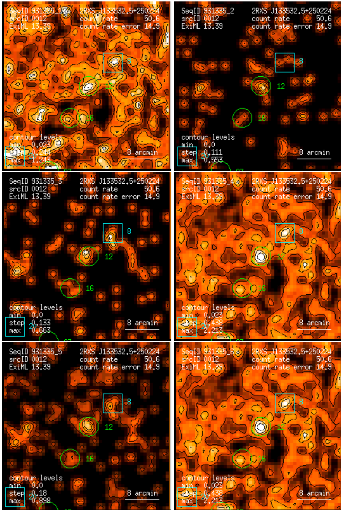
Figure 12: RASS 931335: detection 0012: band rate images, Gaussian filter: (1) PSPC channels 11 – 41, (2) 52 – 90, (3) 91 – 201, (4) 11 – 235, (5) 52 – 201, (6) 11 – 201. Broad band rates in counts/ks. Band rate contour levels in counts/ks/arcmin 2 .
