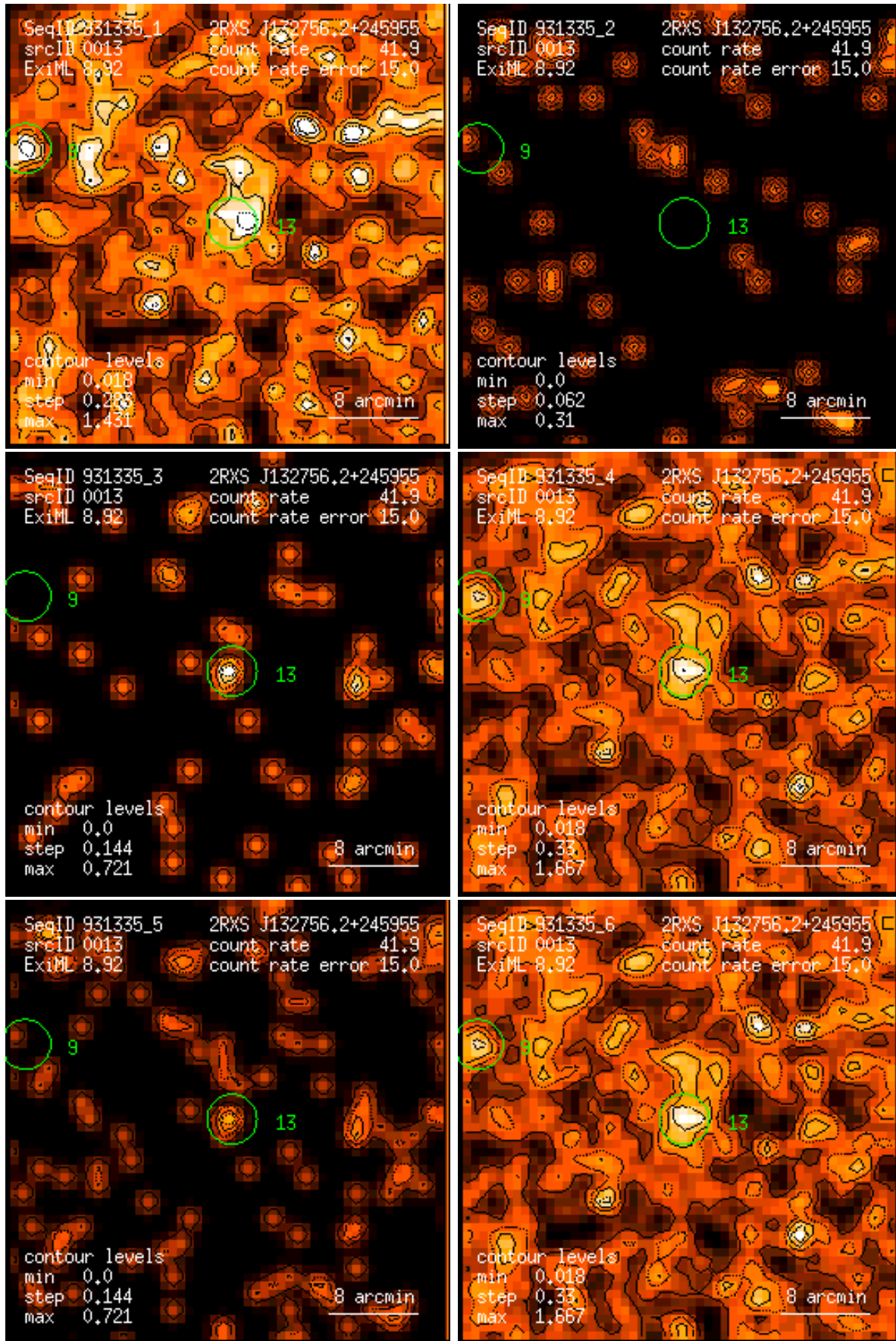
Figure 13: RASS 931335: detection 0013: band rate images, Gaussian filter: (1) PSPC channels 11 – 41, (2) 52 – 90, (3) 91 – 201, (4) 11 – 235, (5) 52 – 201, (6) 11 – 201. Broad band rates in counts/ks. Band rate contour levels in counts/ks/arcmin 2 .
