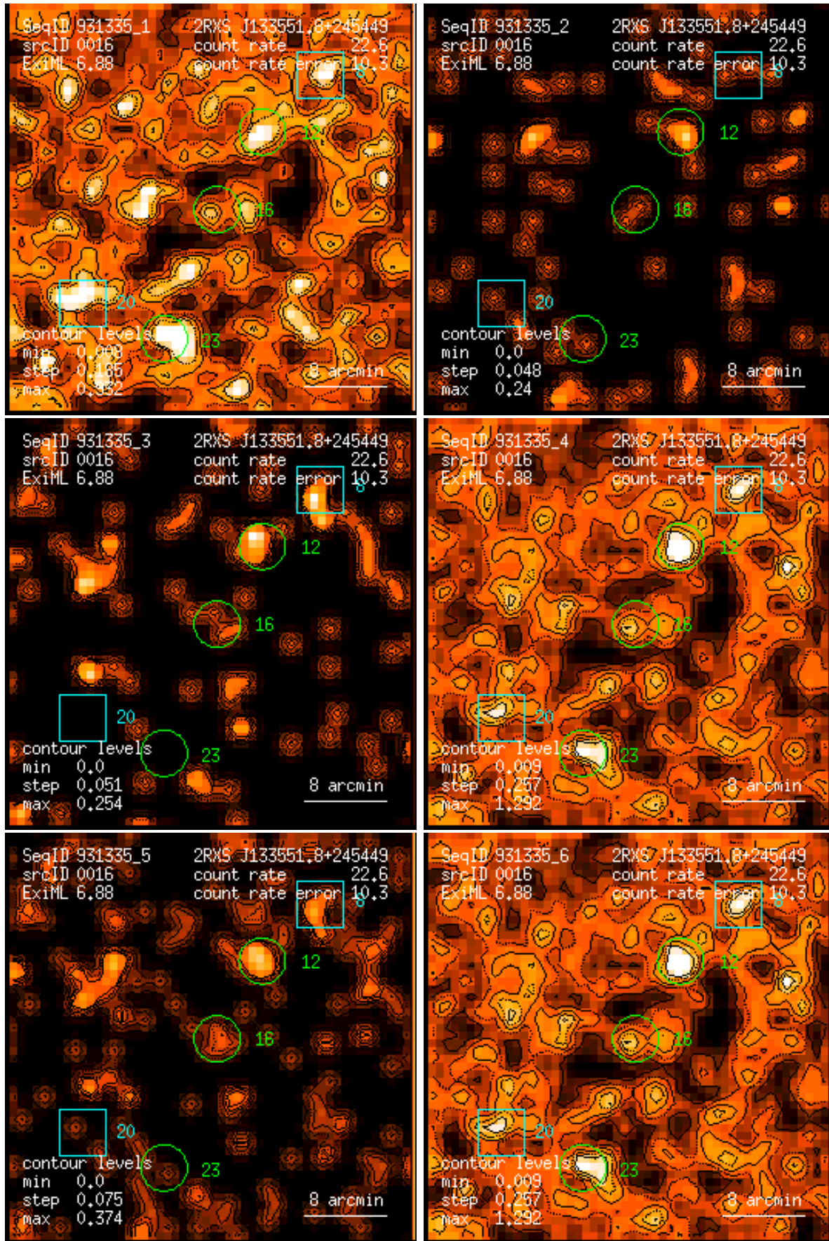
Figure 16: RASS 931335: detection 0016: band rate images, Gaussian filter: (1) PSPC channels 11 – 41, (2) 52 – 90, (3) 91 – 201, (4) 11 – 235, (5) 52 – 201, (6) 11 – 201. Broad band rates in counts/ks. Band rate contour levels in counts/ks/arcmin 2 .
