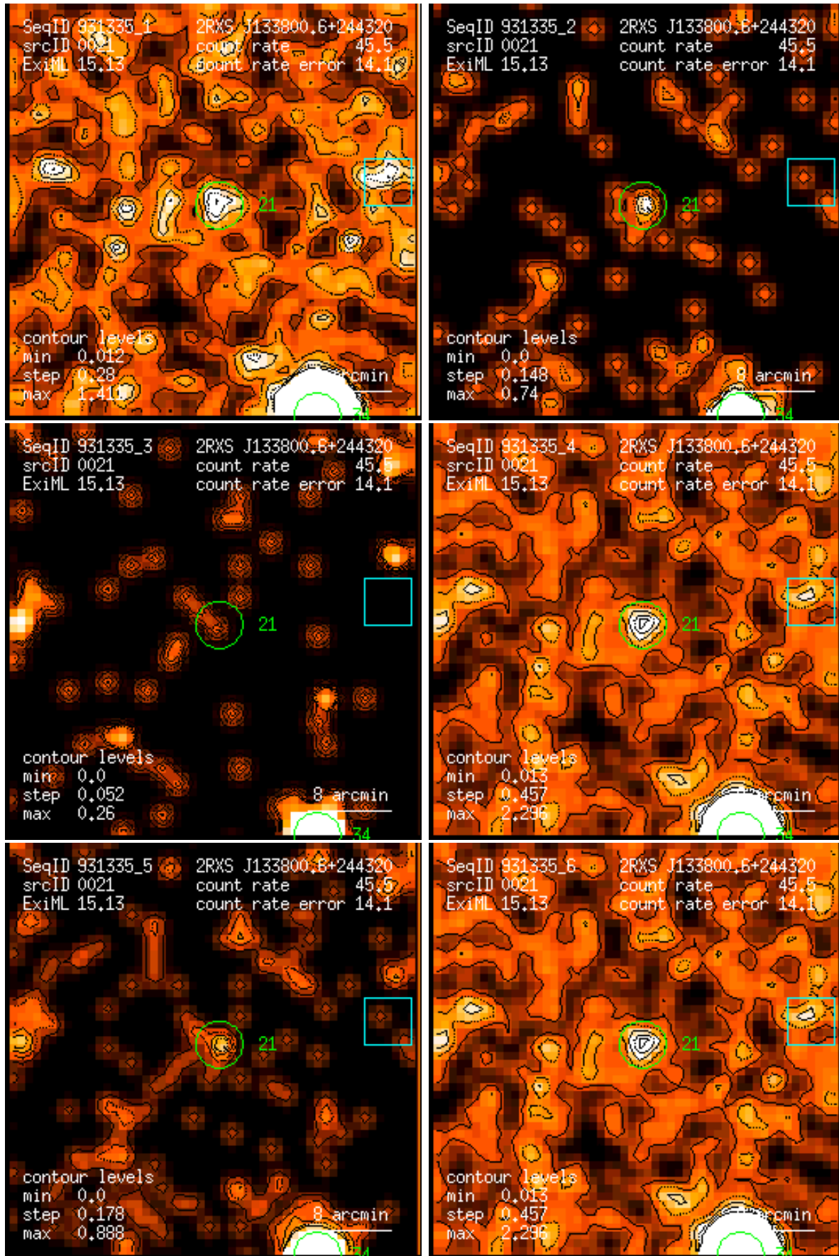
Figure 21: RASS 931335: detection 0021: band rate images, Gaussian filter: (1) PSPC channels 11 – 41, (2) 52 – 90, (3) 91 – 201, (4) 11 – 235, (5) 52 – 201, (6) 11 – 201. Broad band rates in counts/ks. Band rate contour levels in counts/ks/arcmin 2 .
