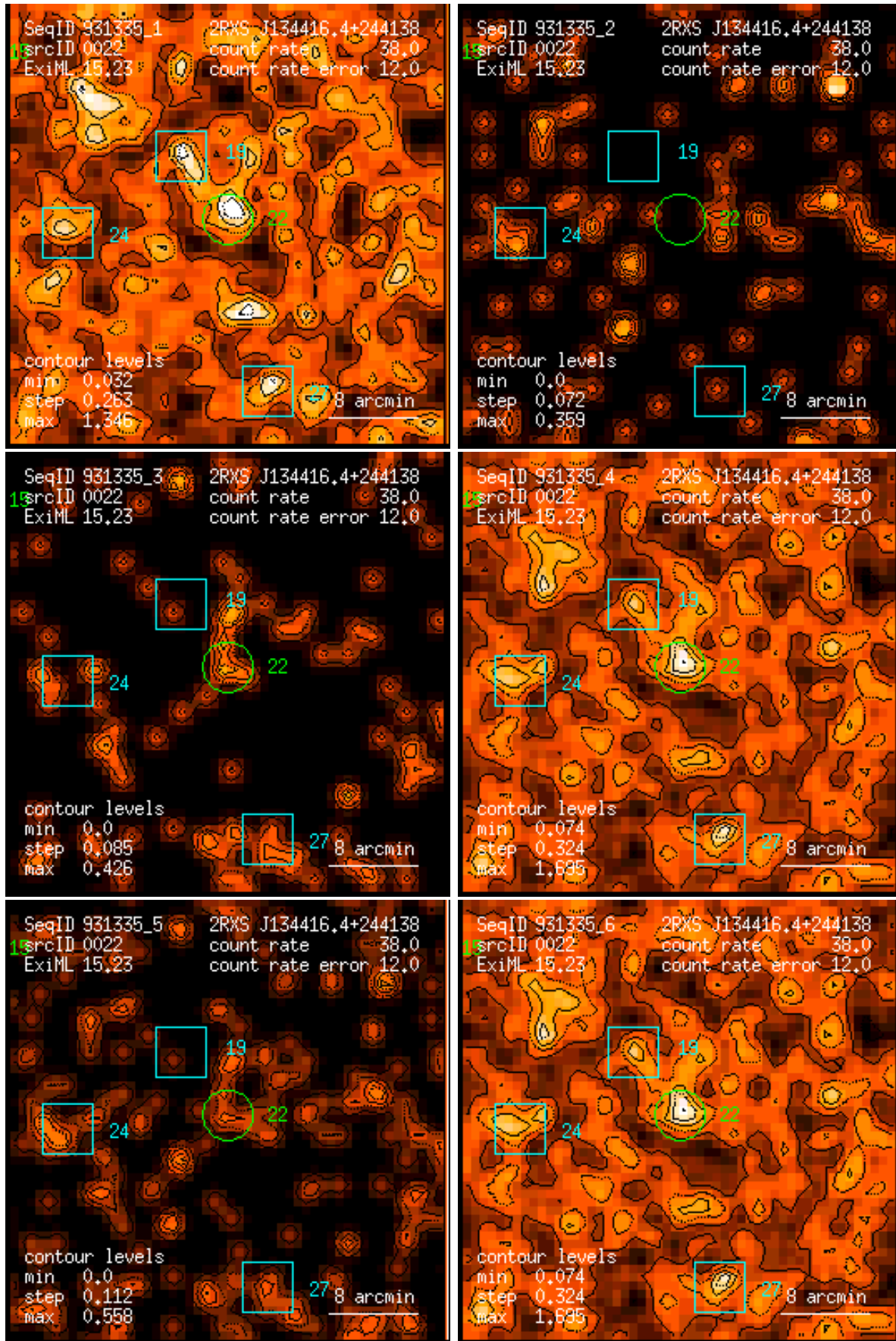
Figure 22: RASS 931335: detection 0022: band rate images, Gaussian filter: (1) PSPC channels 11 – 41, (2) 52 – 90, (3) 91 – 201, (4) 11 – 235, (5) 52 – 201, (6) 11 – 201. Broad band rates in counts/ks. Band rate contour levels in counts/ks/arcmin 2 .
