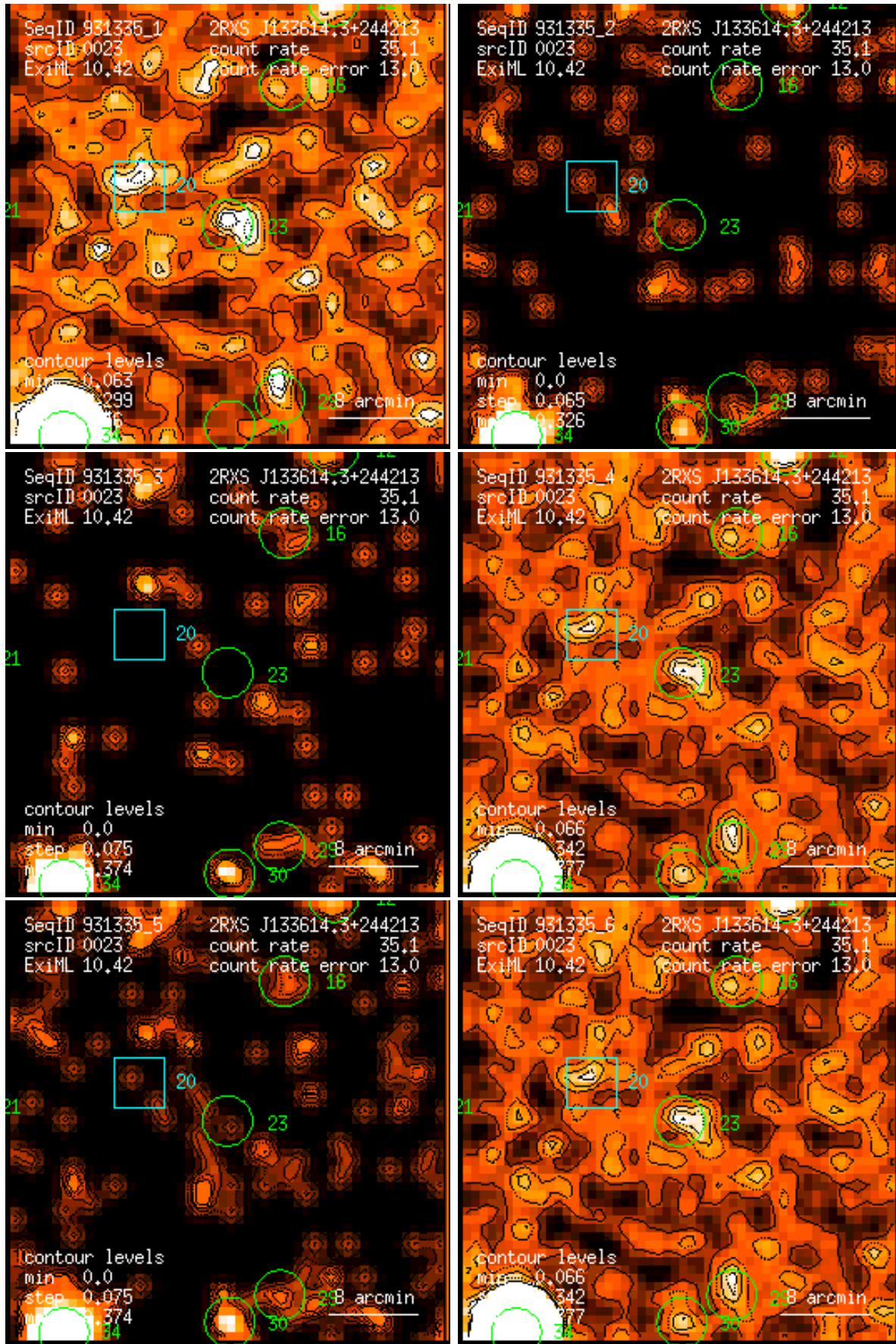
Figure 23: RASS 931335: detection 0023: band rate images, Gaussian filter: (1) PSPC channels 11 – 41, (2) 52 – 90, (3) 91 – 201, (4) 11 – 235, (5) 52 – 201, (6) 11 – 201. Broad band rates in counts/ks. Band rate contour levels in counts/ks/arcmin 2 .
