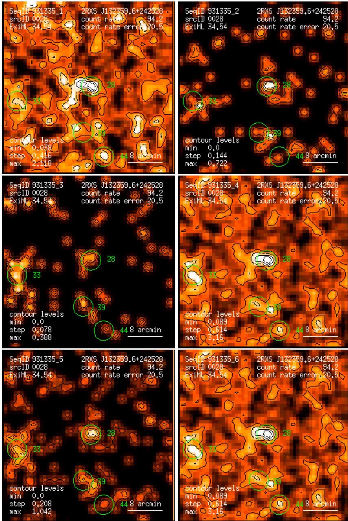
Figure 28: RASS 931335: detection 0028: band rate images, Gaussian filter: (1) PSPC channels 11 – 41, (2) 52 – 90, (3) 91 – 201, (4) 11 – 235, (5) 52 – 201, (6) 11 – 201. Broad band rates in counts/ks. Band rate contour levels in counts/ks/arcmin 2 .
