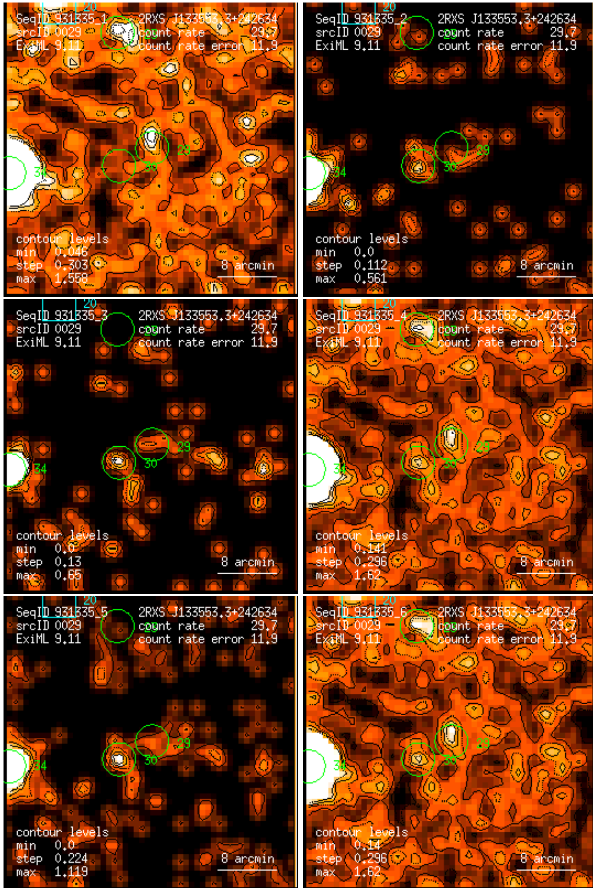
Figure 29: RASS 931335: detection 0029: band rate images, Gaussian filter: (1) PSPC channels 11 – 41, (2) 52 – 90, (3) 91 – 201, (4) 11 – 235, (5) 52 – 201, (6) 11 – 201. Broad band rates in counts/ks. Band rate contour levels in counts/ks/arcmin 2 .
