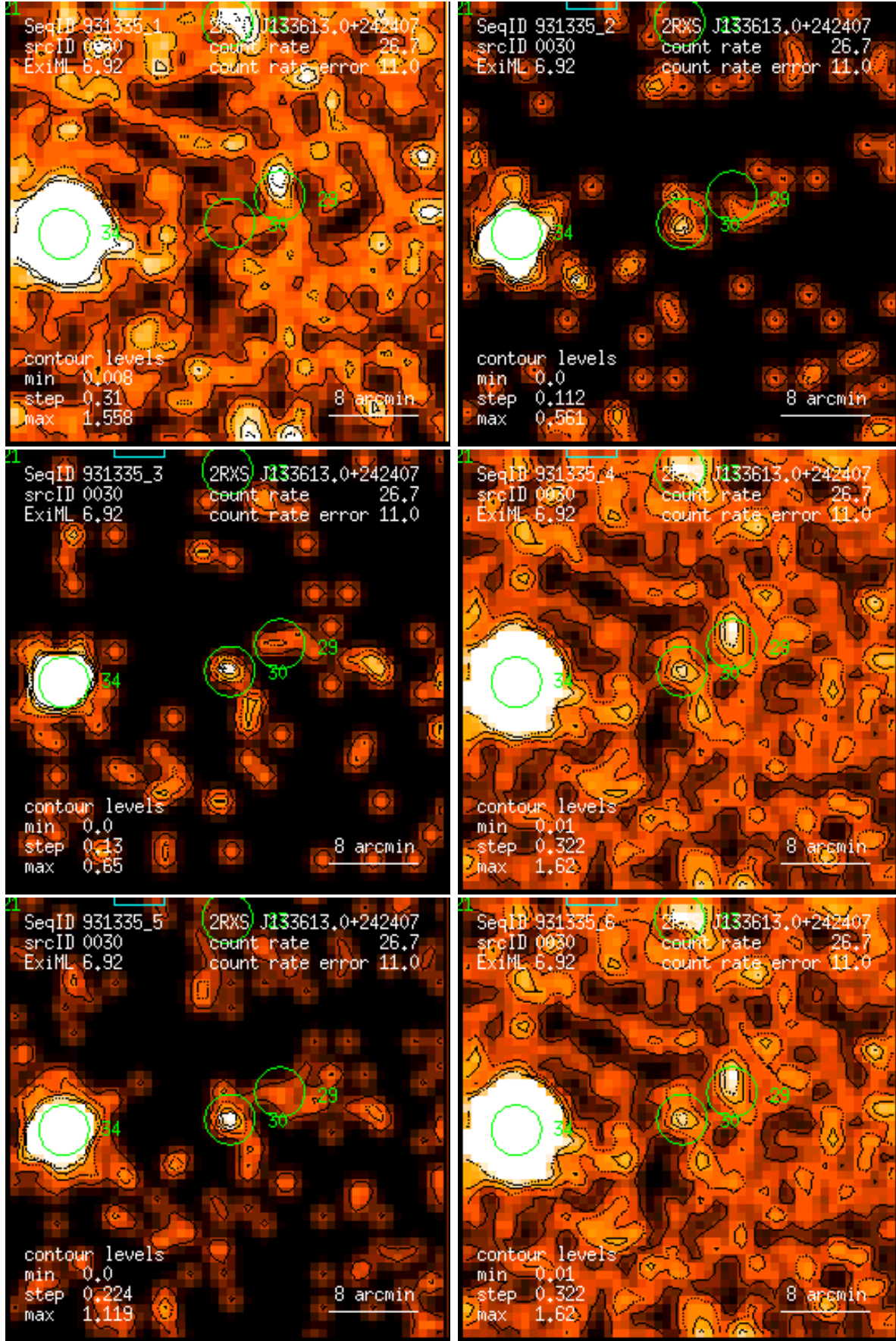
Figure 30: RASS 931335: detection 0030: band rate images, Gaussian filter: (1) PSPC channels 11 – 41, (2) 52 – 90, (3) 91 – 201, (4) 11 – 235, (5) 52 – 201, (6) 11 – 201. Broad band rates in counts/ks. Band rate contour levels in counts/ks/arcmin 2 .
