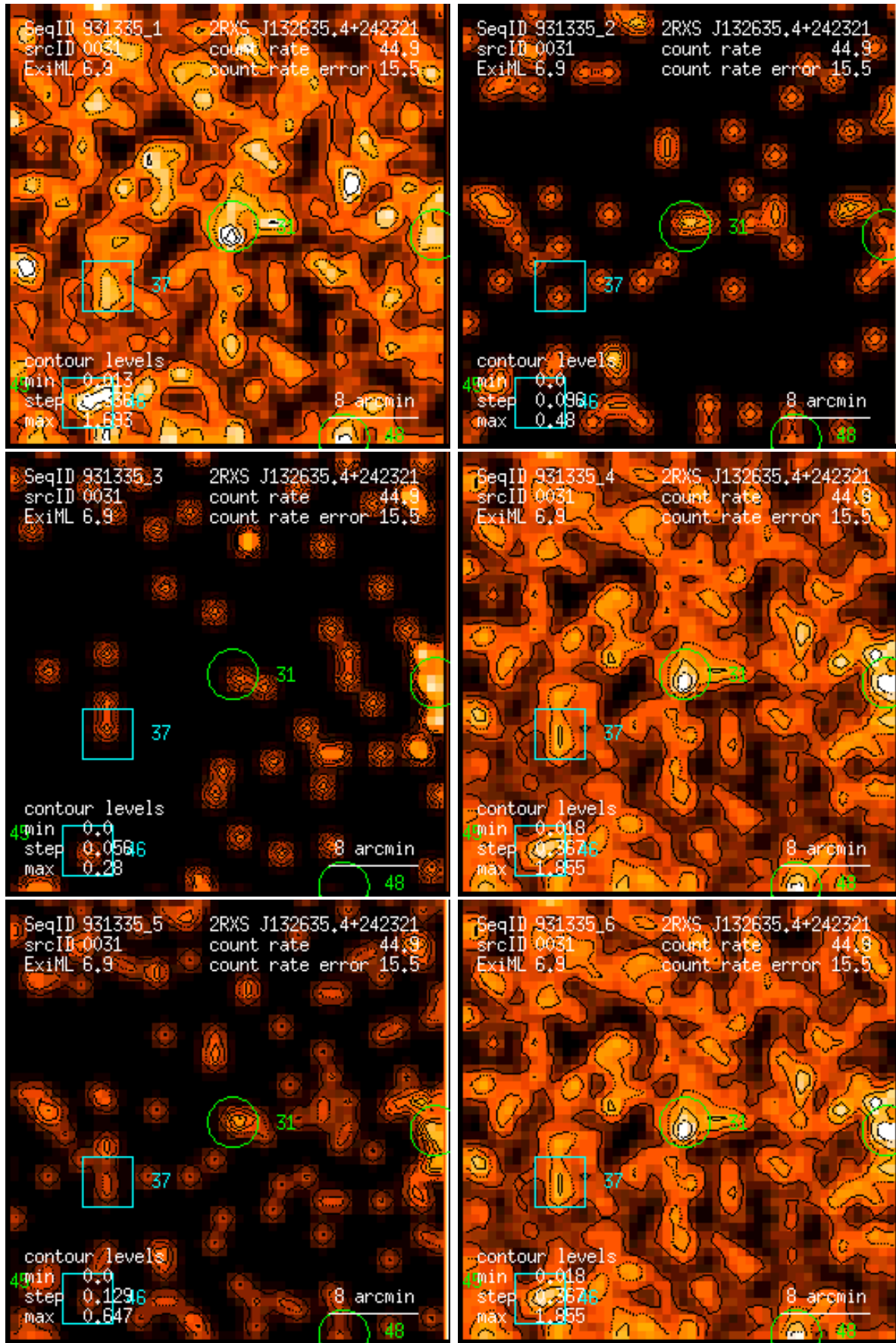
Figure 31: RASS 931335: detection 0031: band rate images, Gaussian filter: (1) PSPC channels 11 – 41, (2) 52 – 90, (3) 91 – 201, (4) 11 – 235, (5) 52 – 201, (6) 11 – 201. Broad band rates in counts/ks. Band rate contour levels in counts/ks/arcmin 2 .
