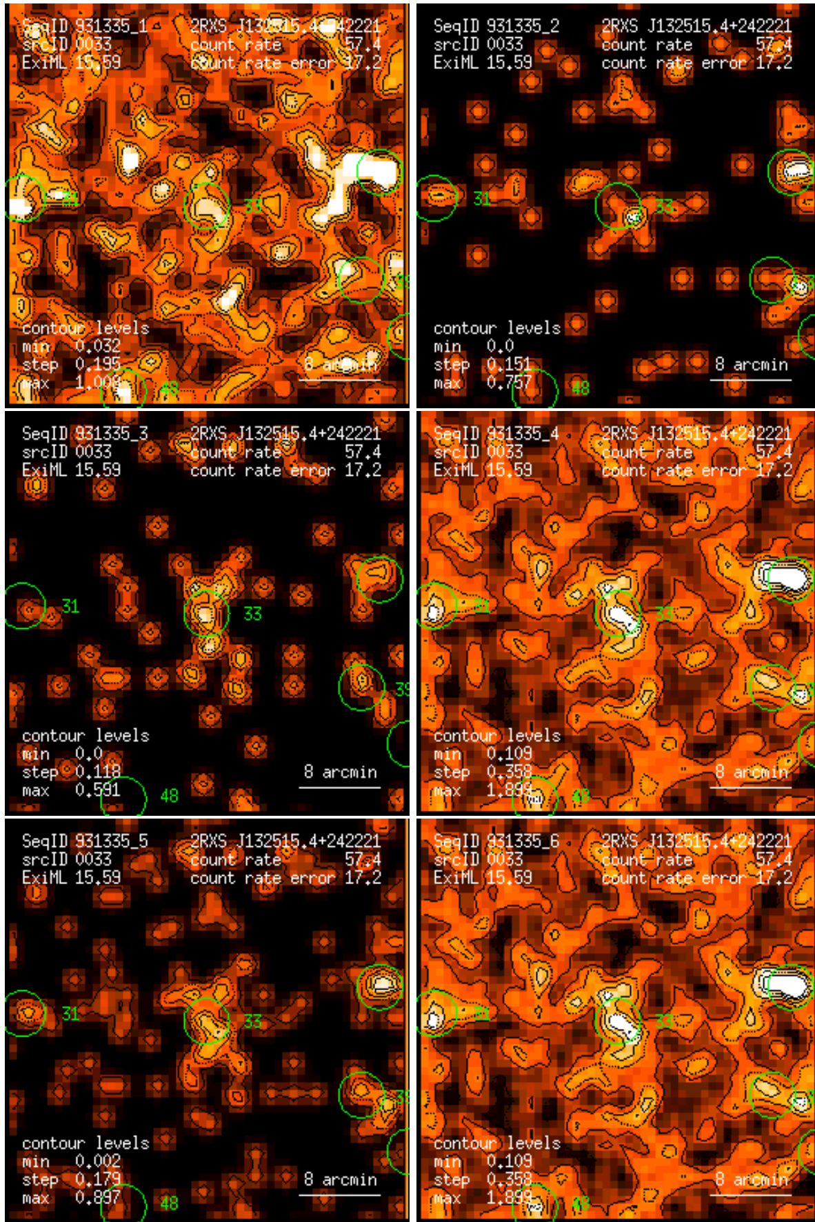
Figure 33: RASS 931335: detection 0033: band rate images, Gaussian filter: (1) PSPC channels 11 – 41, (2) 52 – 90, (3) 91 – 201, (4) 11 – 235, (5) 52 – 201, (6) 11 – 201. Broad band rates in counts/ks. Band rate contour levels in counts/ks/arcmin 2 .
