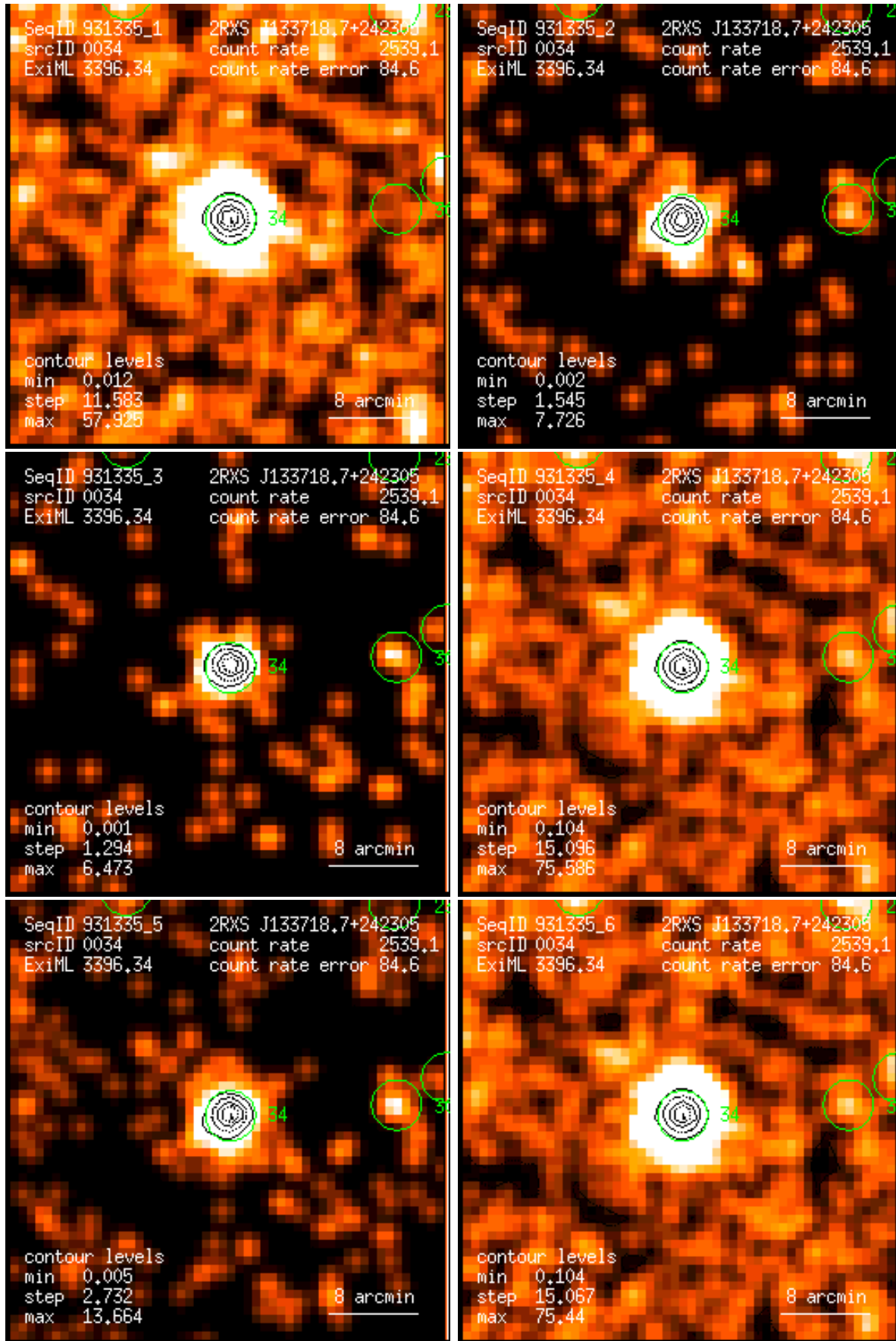
Figure 34: RASS 931335: detection 0034: band rate images, Gaussian filter: (1) PSPC channels 11 – 41, (2) 52 – 90, (3) 91 – 201, (4) 11 – 235, (5) 52 – 201, (6) 11 – 201. Broad band rates in counts/ks. Band rate contour levels in counts/ks/arcmin 2 .
