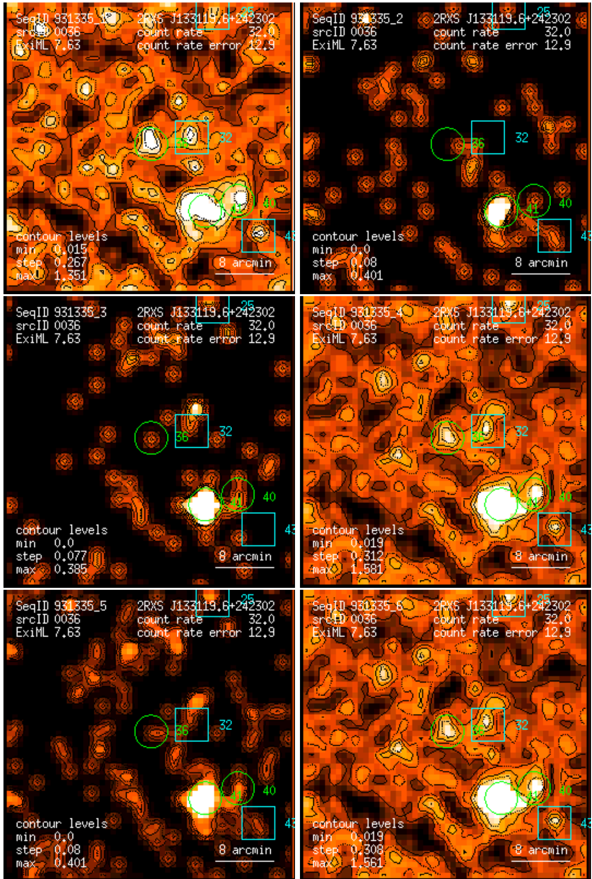
Figure 36: RASS 931335: detection 0036: band rate images, Gaussian filter: (1) PSPC channels 11 – 41, (2) 52 – 90, (3) 91 – 201, (4) 11 – 235, (5) 52 – 201, (6) 11 – 201. Broad band rates in counts/ks. Band rate contour levels in counts/ks/arcmin 2 .
