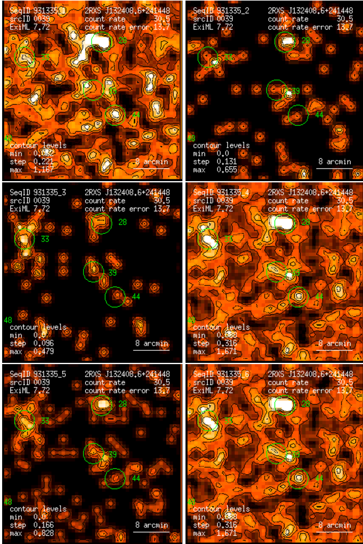
Figure 39: RASS 931335: detection 0039: band rate images, Gaussian filter: (1) PSPC channels 11 – 41, (2) 52 – 90, (3) 91 – 201, (4) 11 – 235, (5) 52 – 201, (6) 11 – 201. Broad band rates in counts/ks. Band rate contour levels in counts/ks/arcmin 2 .
