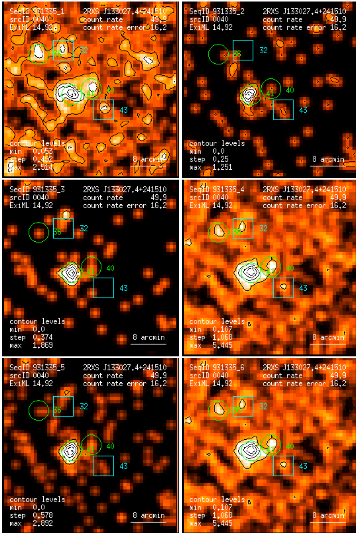
Figure 40: RASS 931335: detection 0040: band rate images, Gaussian filter: (1) PSPC channels 11 – 41, (2) 52 – 90, (3) 91 – 201, (4) 11 – 235, (5) 52 – 201, (6) 11 – 201. Broad band rates in counts/ks. Band rate contour levels in counts/ks/arcmin 2 .
