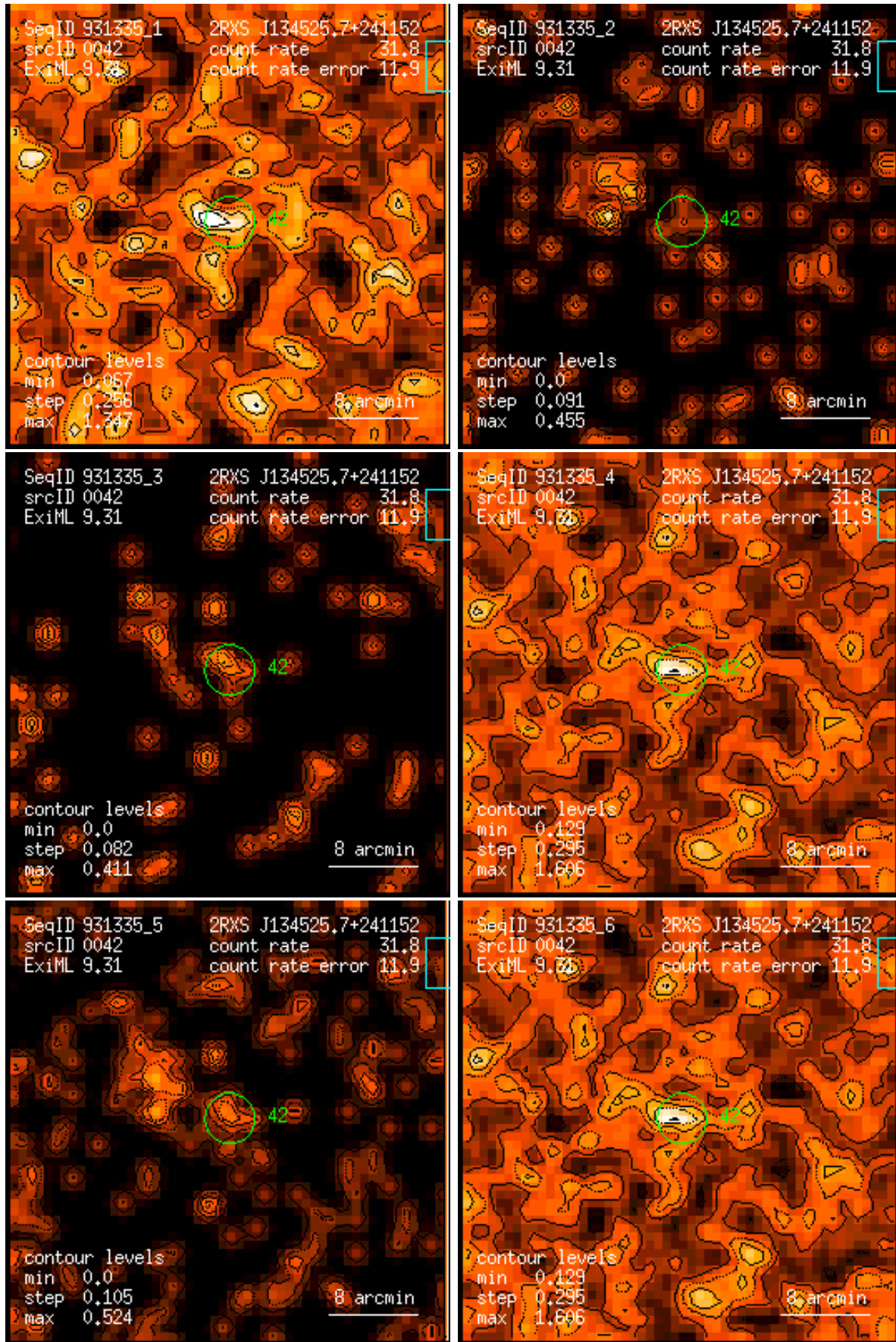
Figure 42: RASS 931335: detection 0042: band rate images, Gaussian filter: (1) PSPC channels 11 – 41, (2) 52 – 90, (3) 91 – 201, (4) 11 – 235, (5) 52 – 201, (6) 11 – 201. Broad band rates in counts/ks. Band rate contour levels in counts/ks/arcmin 2 .
