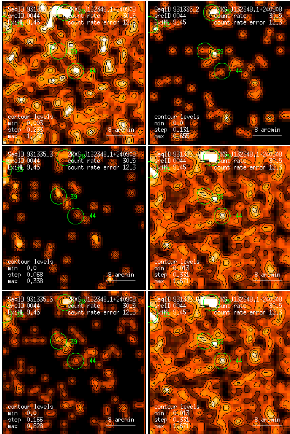
Figure 44: RASS 931335: detection 0044: band rate images, Gaussian filter: (1) PSPC channels 11 – 41, (2) 52 – 90, (3) 91 – 201, (4) 11 – 235, (5) 52 – 201, (6) 11 – 201. Broad band rates in counts/ks. Band rate contour levels in counts/ks/arcmin 2 .
