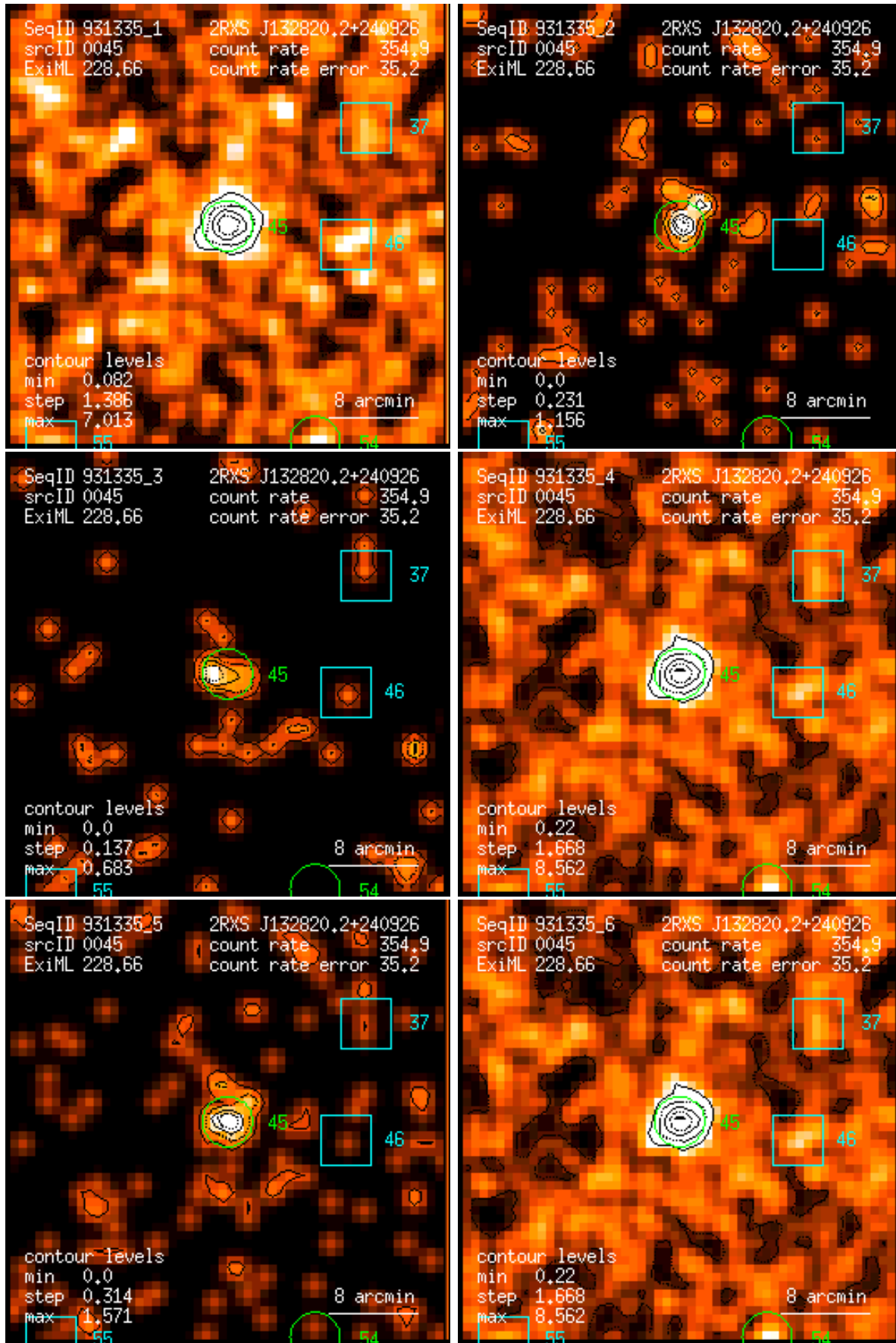
Figure 45: RASS 931335: detection 0045: band rate images, Gaussian filter: (1) PSPC channels 11 – 41, (2) 52 – 90, (3) 91 – 201, (4) 11 – 235, (5) 52 – 201, (6) 11 – 201. Broad band rates in counts/ks. Band rate contour levels in counts/ks/arcmin 2 .
