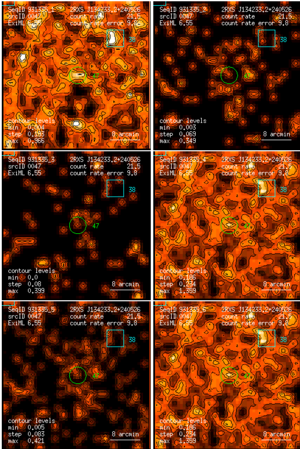
Figure 47: RASS 931335: detection 0047: band rate images, Gaussian filter: (1) PSPC channels 11 – 41, (2) 52 – 90, (3) 91 – 201, (4) 11 – 235, (5) 52 – 201, (6) 11 – 201. Broad band rates in counts/ks. Band rate contour levels in counts/ks/arcmin 2 .
