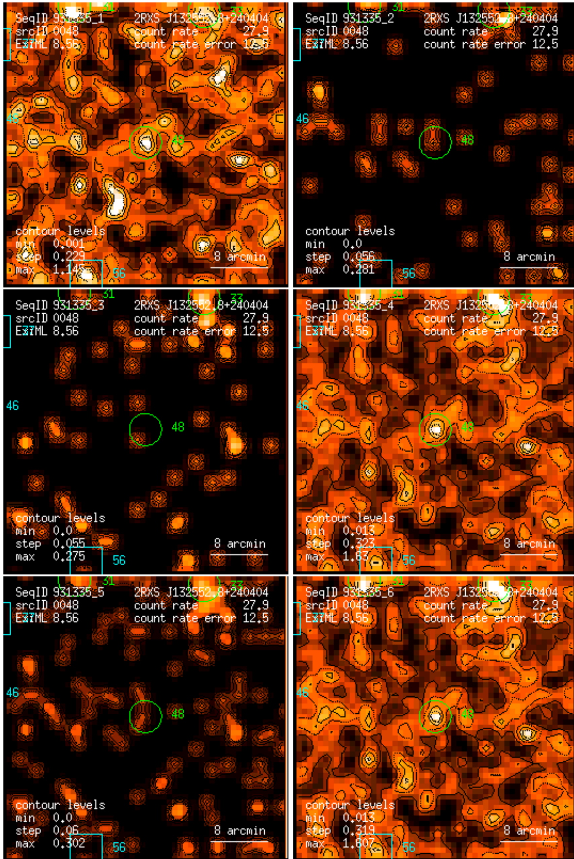
Figure 48: RASS 931335: detection 0048: band rate images, Gaussian filter: (1) PSPC channels 11 – 41, (2) 52 – 90, (3) 91 – 201, (4) 11 – 235, (5) 52 – 201, (6) 11 – 201. Broad band rates in counts/ks. Band rate contour levels in counts/ks/arcmin 2 .
