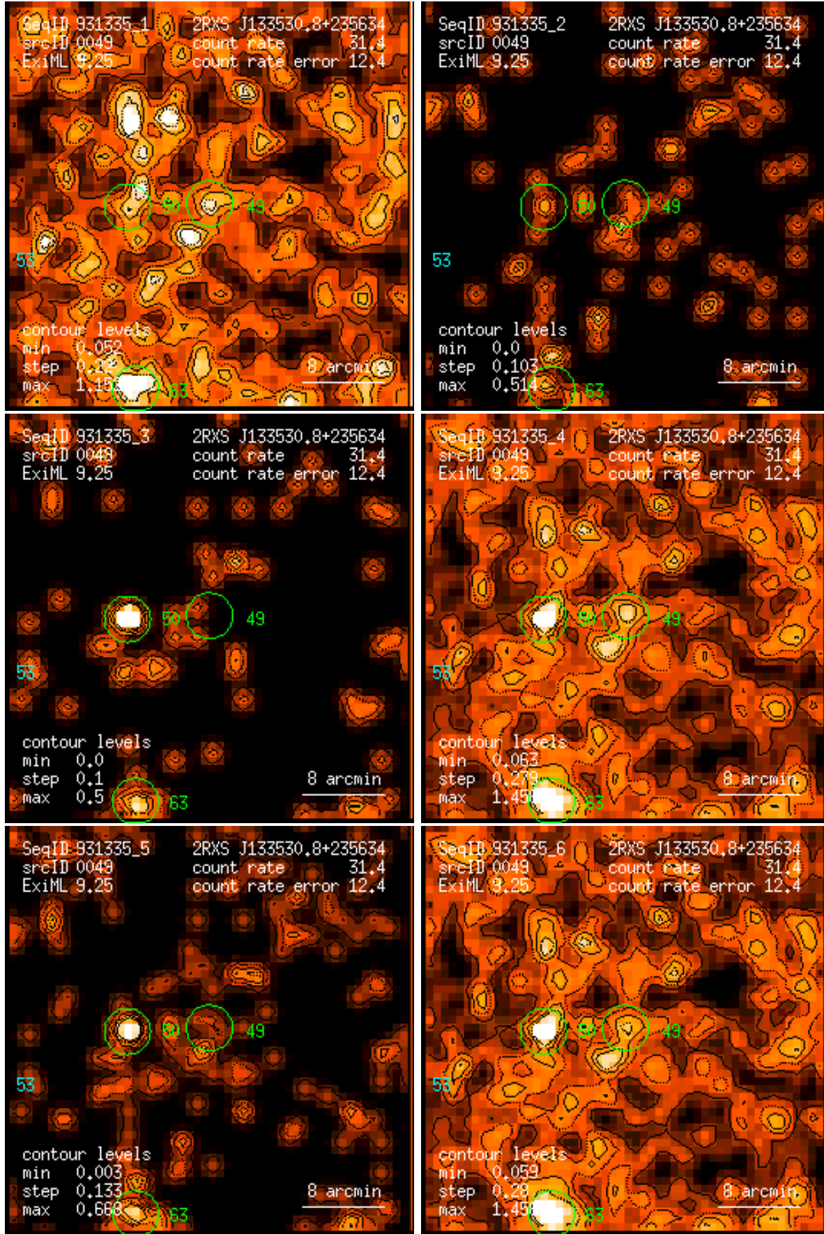
Figure 49: RASS 931335: detection 0049: band rate images, Gaussian filter: (1) PSPC channels 11 – 41, (2) 52 – 90, (3) 91 – 201, (4) 11 – 235, (5) 52 – 201, (6) 11 – 201. Broad band rates in counts/ks. Band rate contour levels in counts/ks/arcmin 2 .
