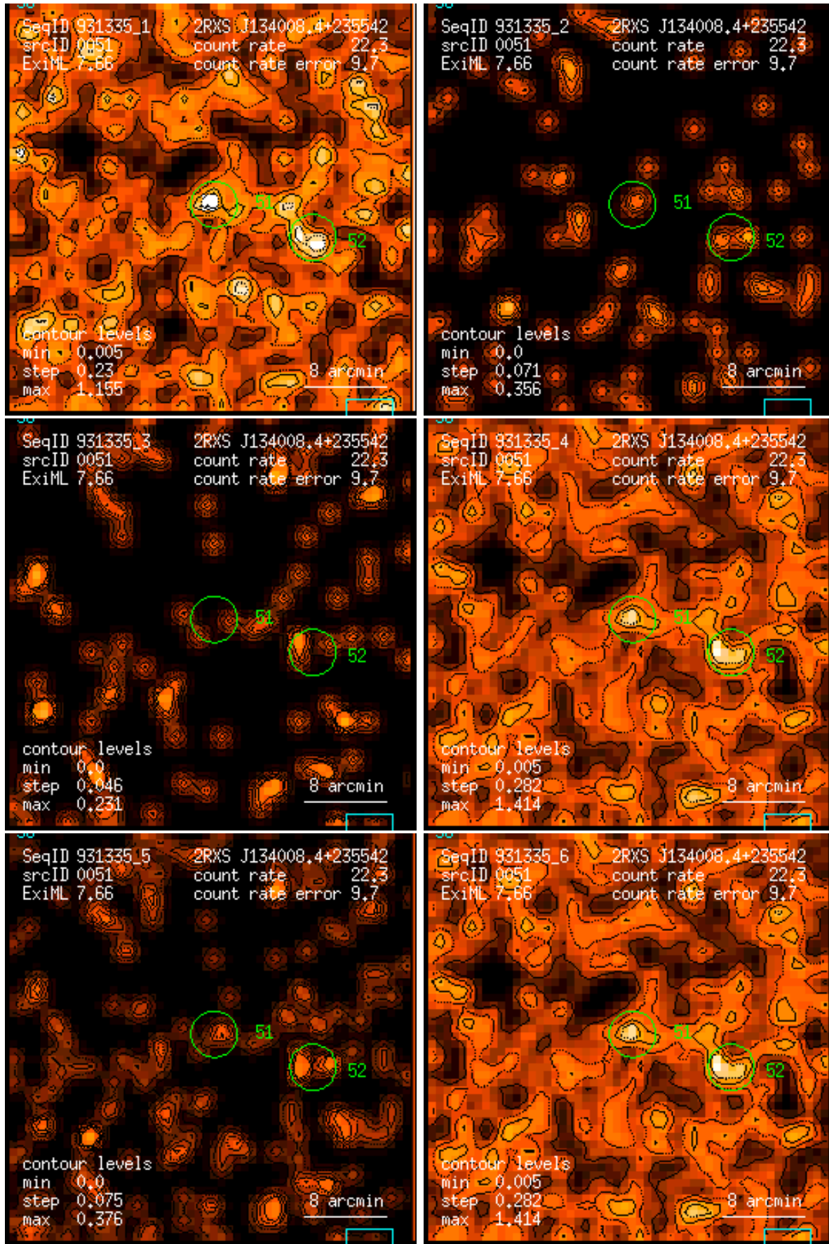
Figure 51: RASS 931335: detection 0051: band rate images, Gaussian filter: (1) PSPC channels 11 – 41, (2) 52 – 90, (3) 91 – 201, (4) 11 – 235, (5) 52 – 201, (6) 11 – 201. Broad band rates in counts/ks. Band rate contour levels in counts/ks/arcmin 2 .
