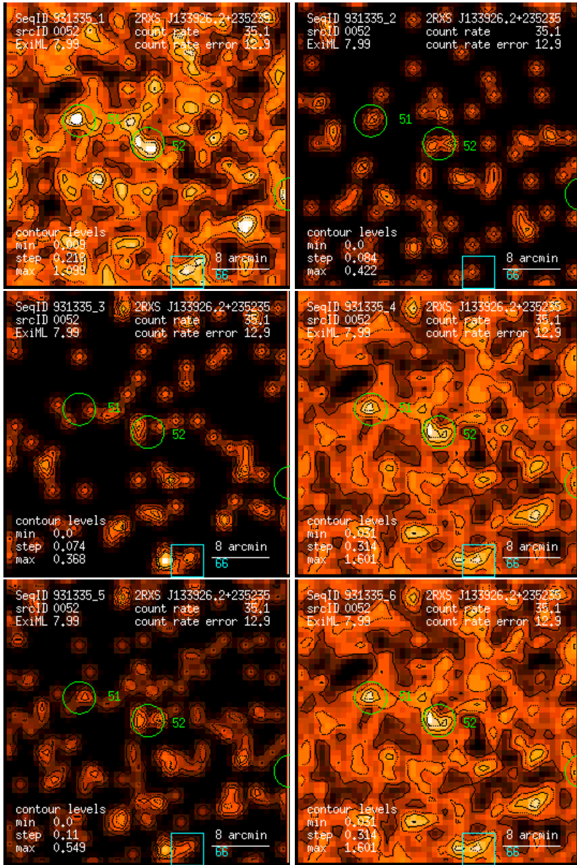
Figure 52: RASS 931335: detection 0052: band rate images, Gaussian filter: (1) PSPC channels 11 – 41, (2) 52 – 90, (3) 91 – 201, (4) 11 – 235, (5) 52 – 201, (6) 11 – 201. Broad band rates in counts/ks. Band rate contour levels in counts/ks/arcmin 2 .
