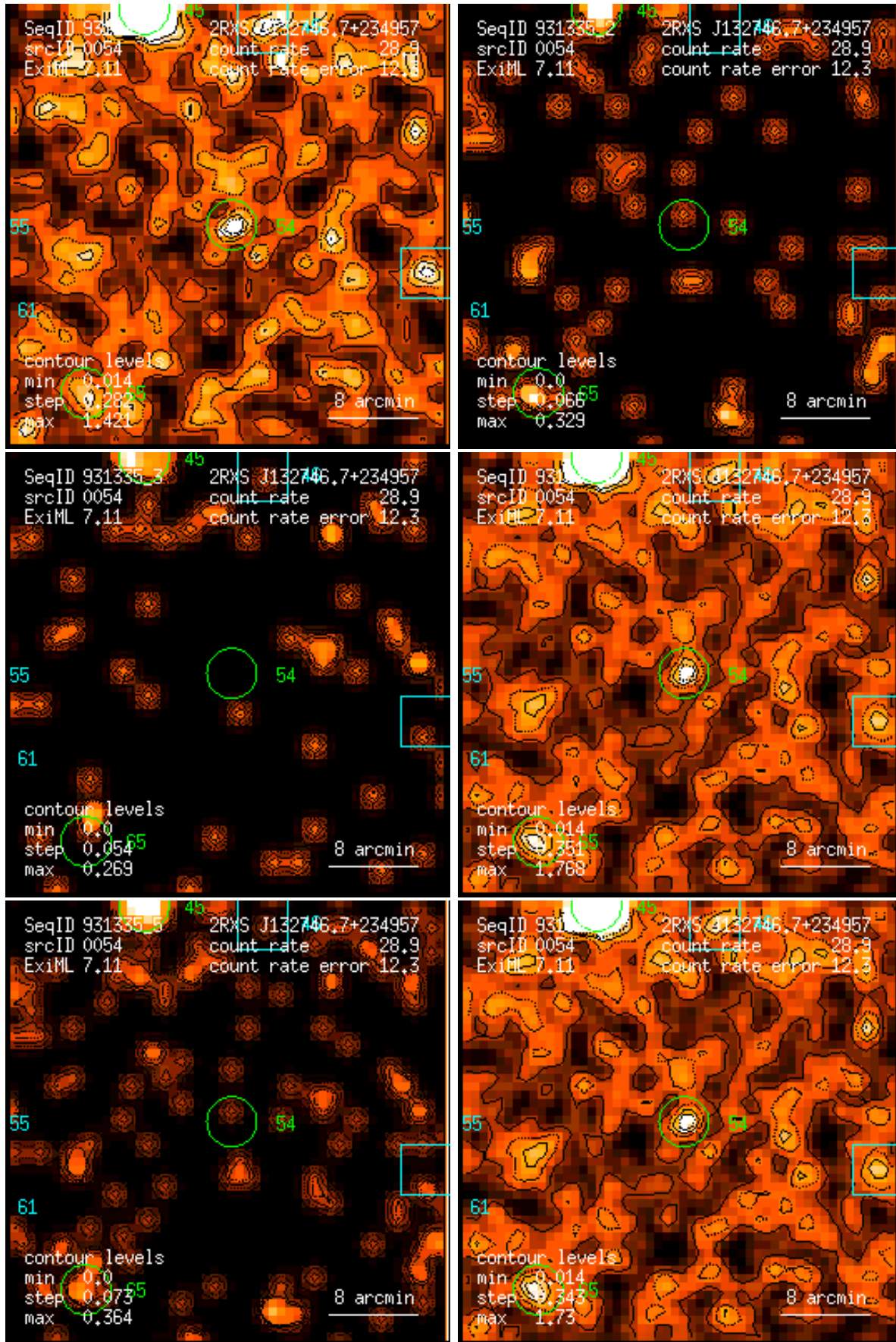
Figure 54: RASS 931335: detection 0054: band rate images, Gaussian filter: (1) PSPC channels 11 – 41, (2) 52 – 90, (3) 91 – 201, (4) 11 – 235, (5) 52 – 201, (6) 11 – 201. Broad band rates in counts/ks. Band rate contour levels in counts/ks/arcmin 2 .
