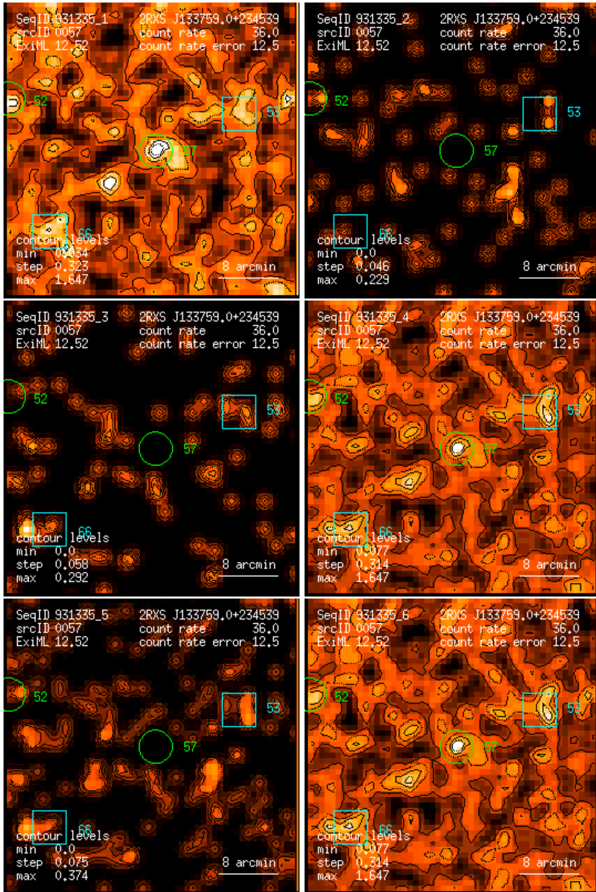
Figure 57: RASS 931335: detection 0057: band rate images, Gaussian filter: (1) PSPC channels 11 – 41, (2) 52 – 90, (3) 91 – 201, (4) 11 – 235, (5) 52 – 201, (6) 11 – 201. Broad band rates in counts/ks. Band rate contour levels in counts/ks/arcmin 2 .
