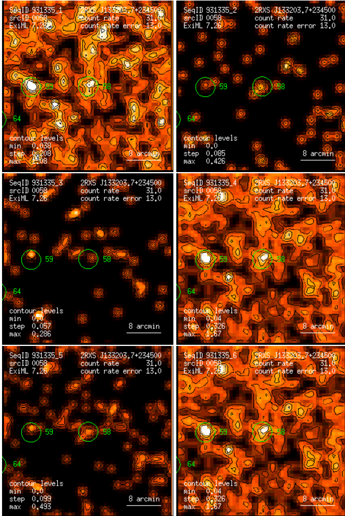
Figure 58: RASS 931335: detection 0058: band rate images, Gaussian filter: (1) PSPC channels 11 – 41, (2) 52 – 90, (3) 91 – 201, (4) 11 – 235, (5) 52 – 201, (6) 11 – 201. Broad band rates in counts/ks. Band rate contour levels in counts/ks/arcmin 2 .
