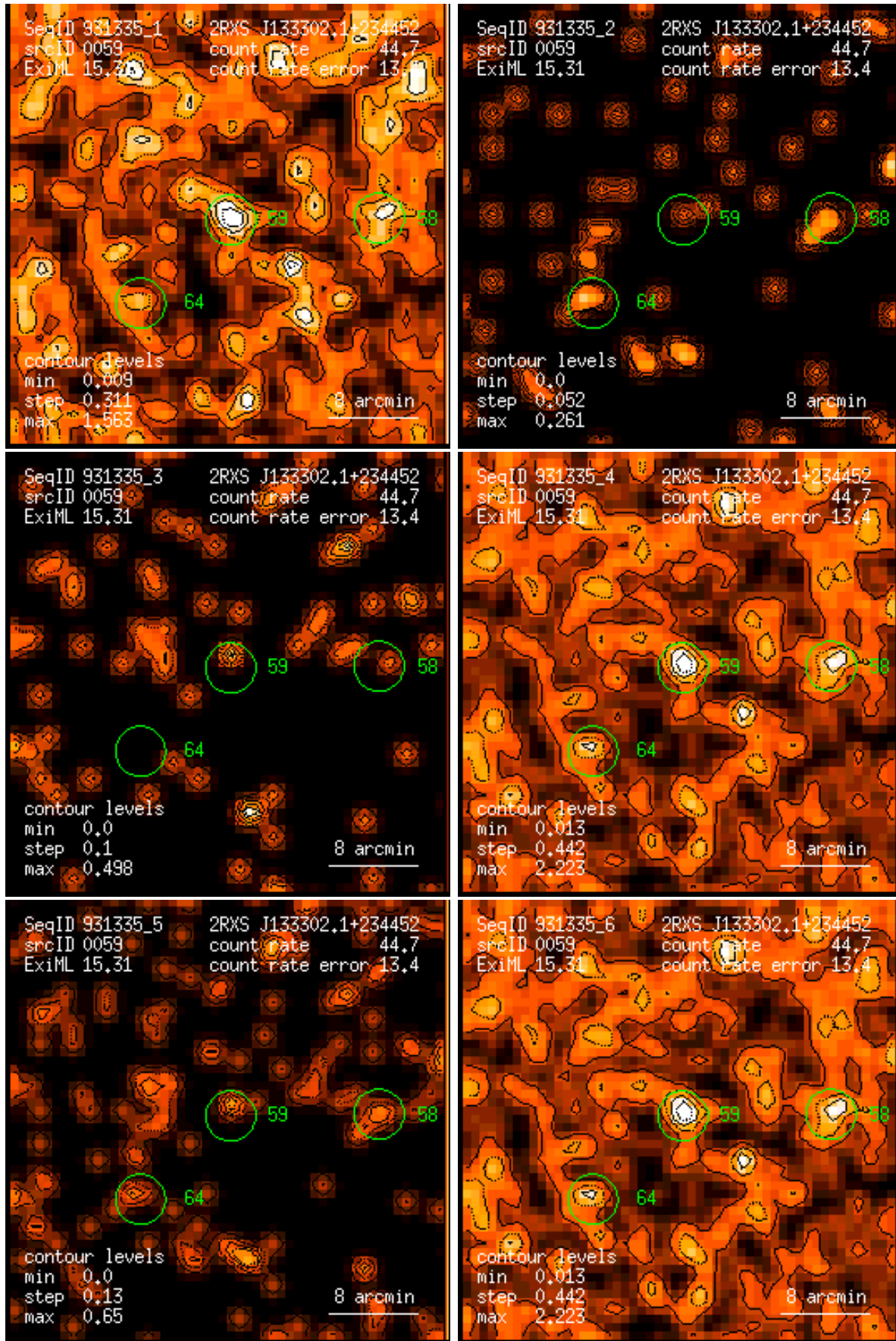
Figure 59: RASS 931335: detection 0059: band rate images, Gaussian filter: (1) PSPC channels 11 – 41, (2) 52 – 90, (3) 91 – 201, (4) 11 – 235, (5) 52 – 201, (6) 11 – 201. Broad band rates in counts/ks. Band rate contour levels in counts/ks/arcmin 2 .
