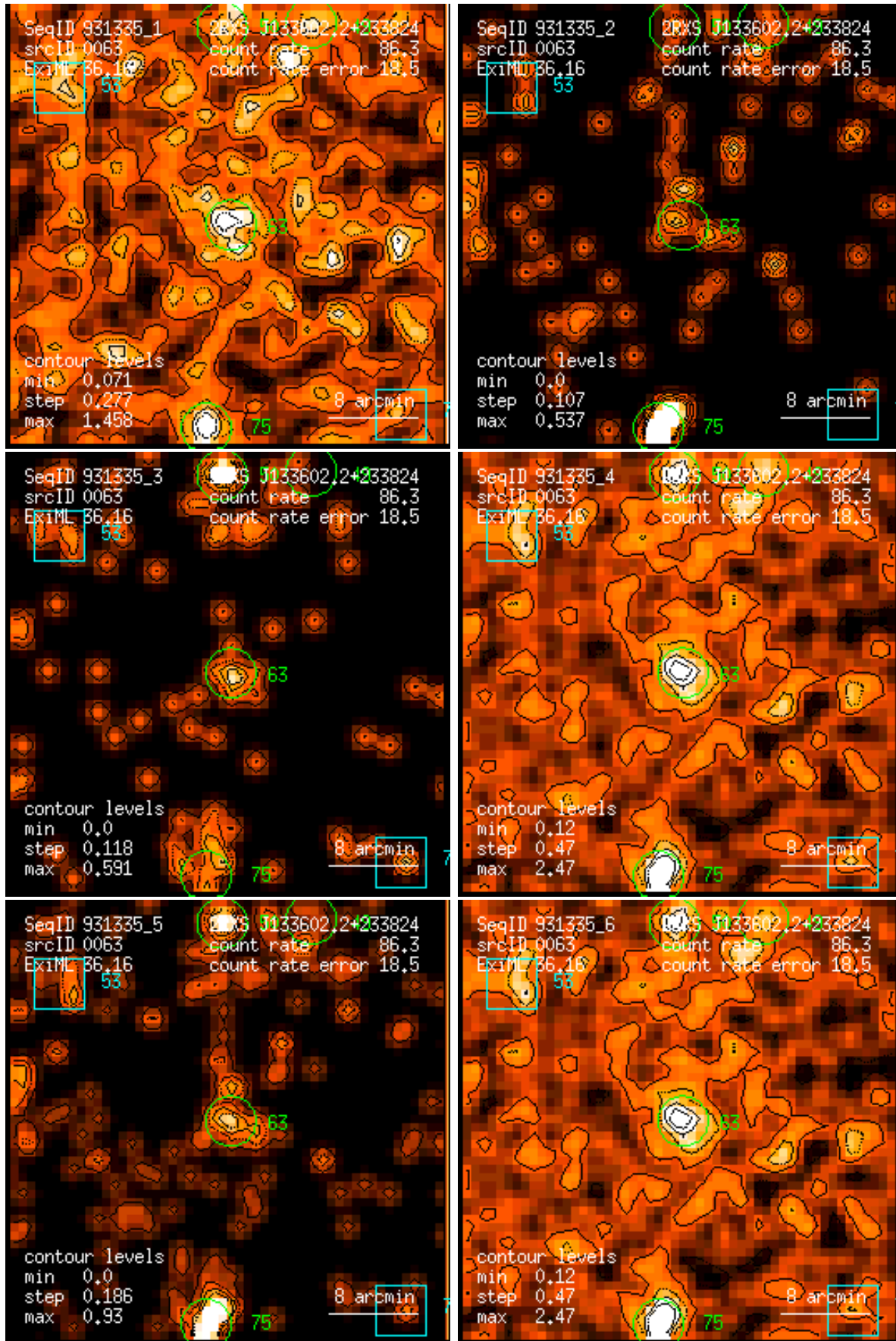
Figure 63: RASS 931335: detection 0063: band rate images, Gaussian filter: (1) PSPC channels 11 – 41, (2) 52 – 90, (3) 91 – 201, (4) 11 – 235, (5) 52 – 201, (6) 11 – 201. Broad band rates in counts/ks. Band rate contour levels in counts/ks/arcmin 2 .
