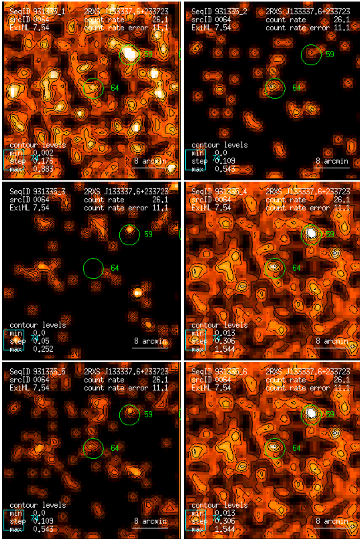
Figure 64: RASS 931335: detection 0064: band rate images, Gaussian filter: (1) PSPC channels 11 – 41, (2) 52 – 90, (3) 91 – 201, (4) 11 – 235, (5) 52 – 201, (6) 11 – 201. Broad band rates in counts/ks. Band rate contour levels in counts/ks/arcmin 2 .
